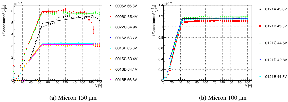
Figure 8: CV of Micron sensors with two active thicknesses. The V_{dep} obtained from each CV curve is written in the legend, and the required limit is indicated by the dashed red lines.
