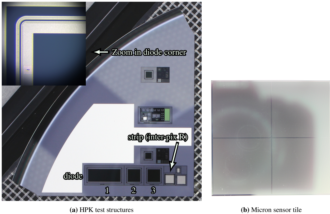
Figure 3: HPK TS with zoom-in photo of a diode, and a Micron sensor tile. The sizes between the TS die and the sensor tile is not to the actual proportion.
