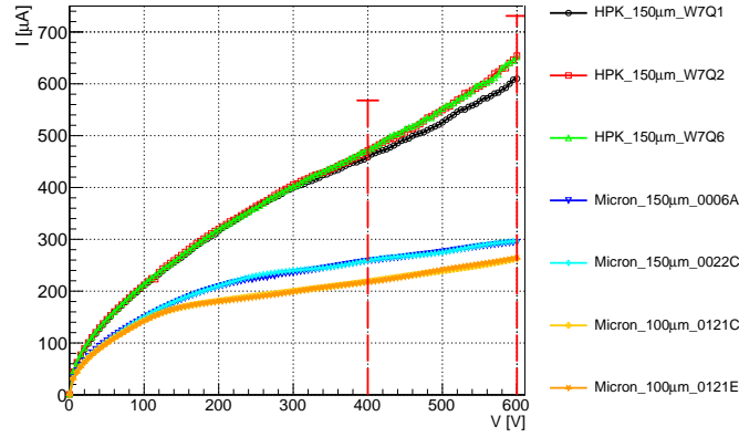
Figure 6: IV curves of irradiated sensor tiles. All the measurements are within specification, as indicated by the dashed red lines: the limit on I is at 400 V for 100 \mu\text{m} sensors and at 600 V for 150 \mu\text{m} sensors, the short horizontal lines on the top of the dashed lines indicate the I limit calculated using the default size of quad sensor tiles.
