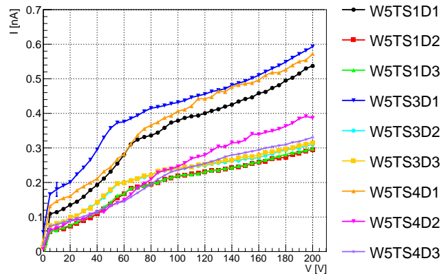
Figure 5: IV of nine un-irradiated HPK diodes from wafer 5. Diodes on three TS dies were tested, on each die there are three diodes, the diodes labelled D1 are of size 5 \times 10 \text{ mm}^2 , D2 and D3 are of size 5 \times 5 \text{ mm}^2 .
