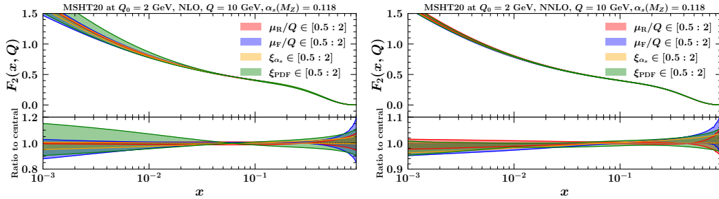
Figure 1 – The structure function F_2 from Ref. 8 versus x , at NLO and NNLO in perturbation theory, with the uncertainty bands associated with variations of renormalization and factorization scales, \mu_R and \mu_F , and resummation scale parameters \xi_{\alpha_s} and \xi_{\text{PDF}} . We use MSHT20 PDFs at Q_0 = 2 GeV and \alpha_s(M_Z) = 0.118 as RGE inputs.
