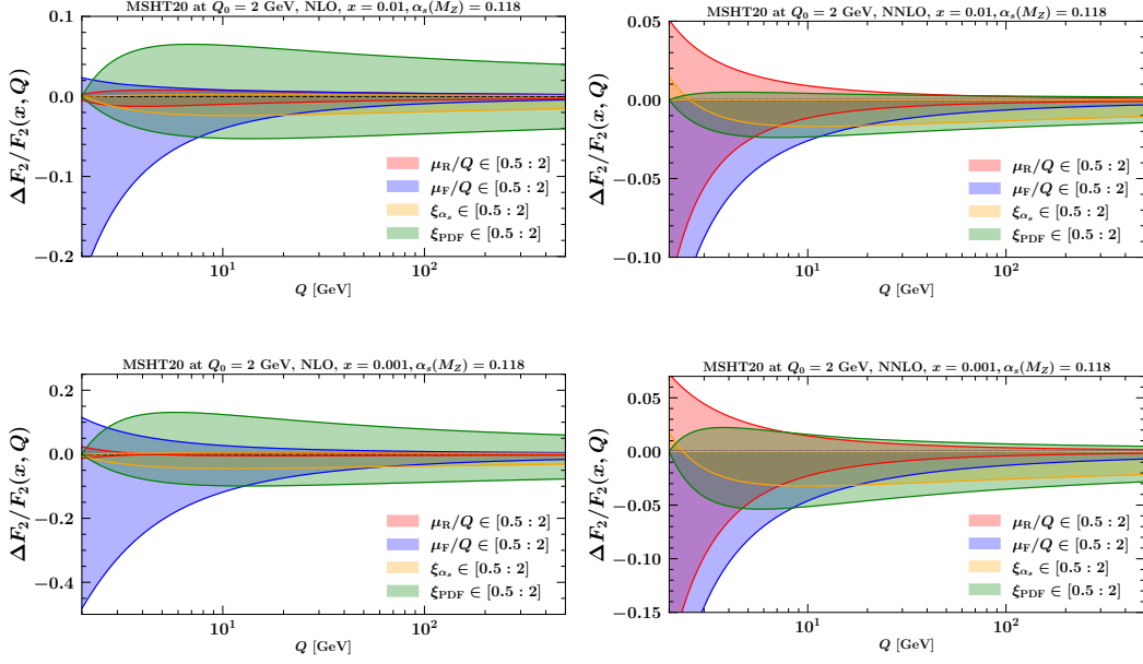
Figure 2 – Q -dependence of the relative variation \Delta F_2/F_2 for x = 10^{-2} (top) and x = 10^{-3} (bottom), at NLO (left) and NNLO (right), associated with variations of renormalization and factorization scales, \mu_R and \mu_F , and resummation scale parameters \xi_{\alpha_s} and \xi_{\text{PDF}} .
