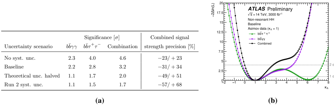
Figure 3: (a) The projected significance and the precision on the measured signal strength in the SM hypothesis shown for four uncertainty scenarios. (b) Likelihood distributions as a function of \kappa_\lambda for the HH \rightarrow b\bar{b}\tau^+\tau^- , HH \rightarrow b\bar{b}\gamma\gamma and their combination. For more details see [8]
