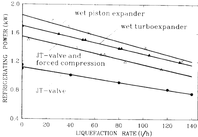
Figure 5. Characteristics of the refrigerator/liquefier
