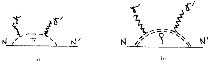
Fig.1. A few diagrams representing the Compton effect on the nucleon
