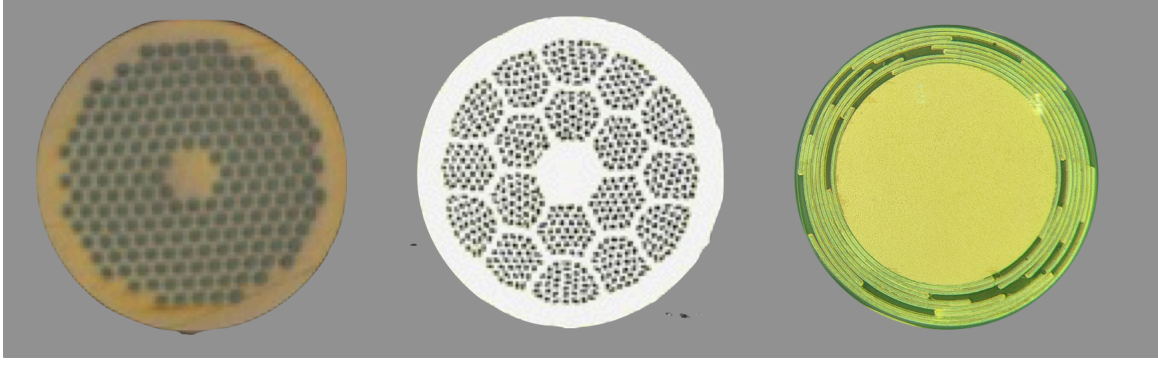
Figure 7: Cross-sections, not in scale, of \text{Nb}_3\text{Sn} (left, 0.85 mm \varnothing ), and Bi2212 (center, 0.8 mm \varnothing ) composite wires produced by Bruker-OST, and a REBCO CORC ® wire (right, 3.4 mm \varnothing ) by ACT LLC.
