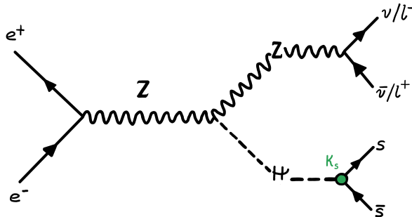
Figure 2: Tree-level Feynman diagram for production of a Higgs boson in association with a Z boson. The Higgs decays hadronically to strange quarks (with Yukawa coupling strength modifier \kappa_s ) and the Z decays leptonically to charged leptons or neutrinos. Drawing by F. Cairo.
