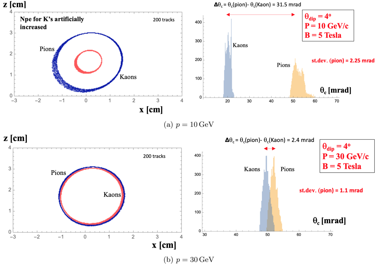
Figure 35: Smearing effect in the SiD/ILD RICH for \theta_{\text{dip}} = 4^\circ , B = 5 \text{ T} , and L = 25 \text{ cm} . Cherenkov rings are imaged in the detector plane and plots of all 2D-hits, \{x_{\text{final}}[i], z_{\text{final}}[i]\} , with no cuts and no fitting are shown for (a) p = 10 \text{ GeV} and (b) p = 30 \text{ GeV} .
