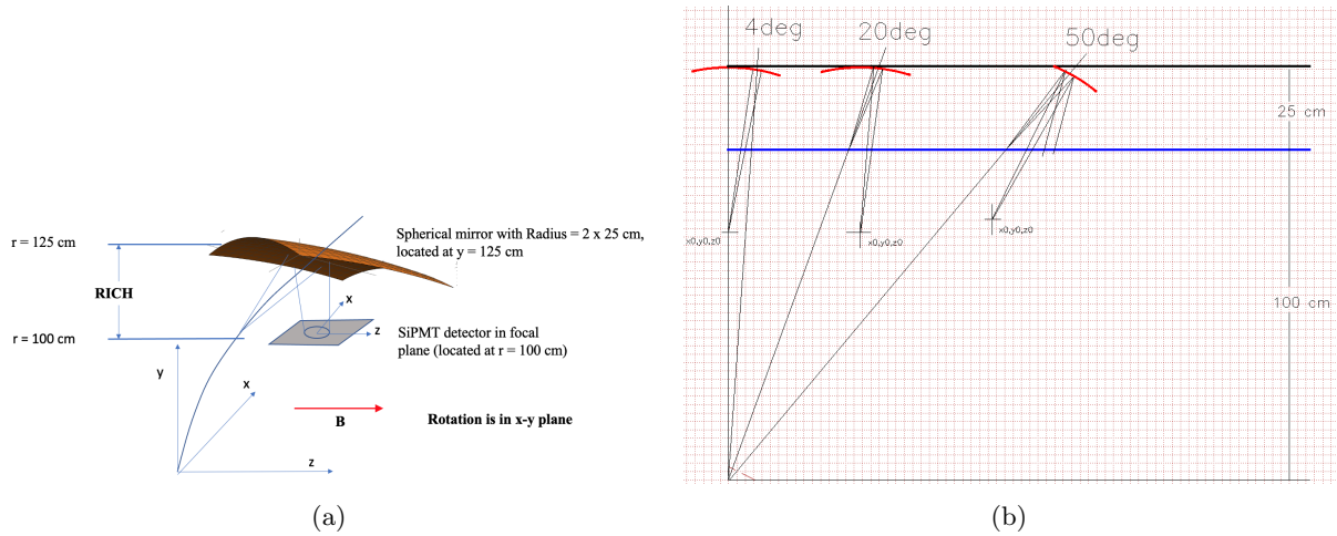
Figure 31: (a) A schematic diagram of the helix trajectory and Cherenkov cone. Notice that cones move in 3D. A simple program was implemented: step through the magnetic field, radiate Cherenkov photons when 100 < r < 125 \text{ cm} , reflect them from a spherical mirror, and find their intersection with a detector plane. (b) Ray tracing model for the simulation of three dip angles.
