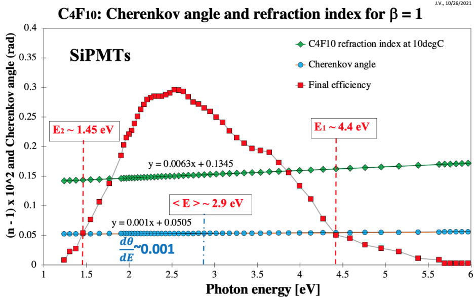
Figure 28: Final efficiency for the SiPM design: the C_4F_{10} refraction index plotted as a function of photon energy.
