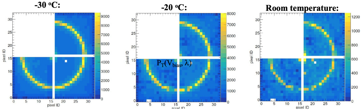
Figure F1: SiPM thermal random noise in images of Cherenkov rings as a function of temperature. These are results from EIC detector R&D [104]. We are proposing to run the SiPMs at 1–2 °C and to eliminate the thermal noise by a timing cut.
