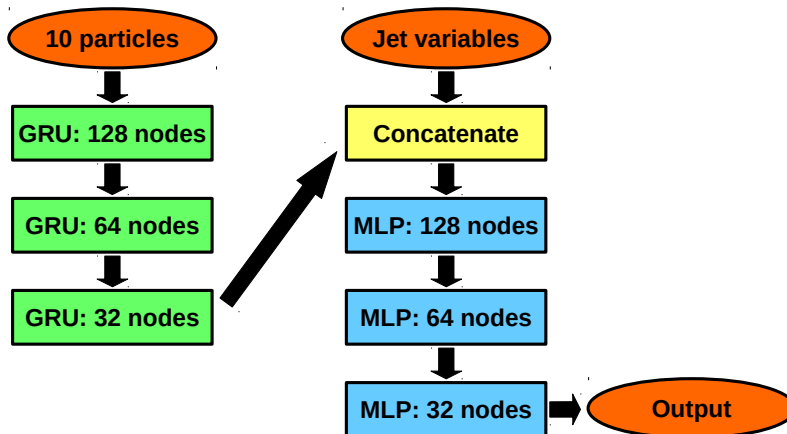
Figure 4: A cartoon of the network architecture used for the jet flavour tagger ANN. The arrows denote the flow of vectors through the network.
