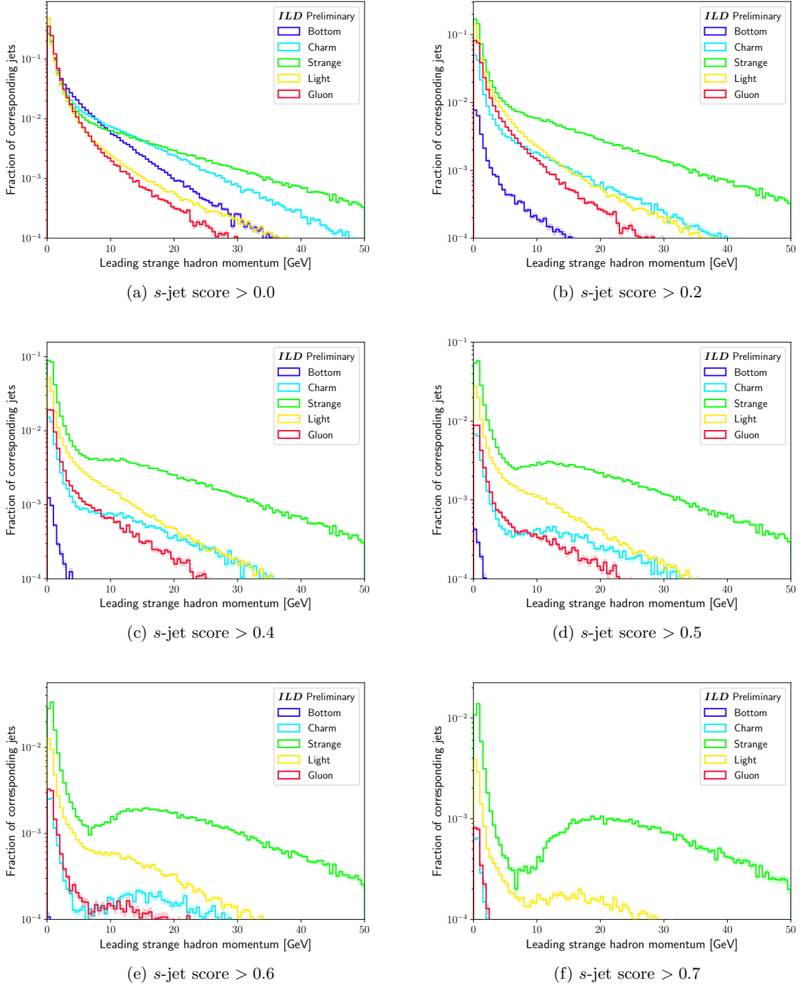
Figure 8: Distributions of the momentum of the leading strange particle in jets from h(\rightarrow q\bar{q}/gg)Z(\rightarrow \nu\bar{\nu}) events. The distributions are shown for different choices of cut on s -jet score of the described jet flavour tagger, Eq. 5. The momentum of the leading strange particle is determined by following the same procedure as for Fig. 3. The sum-of-weights for each class is normalised to 1 in (a) but is not renormalised following the application of cuts in (b) through (e).
