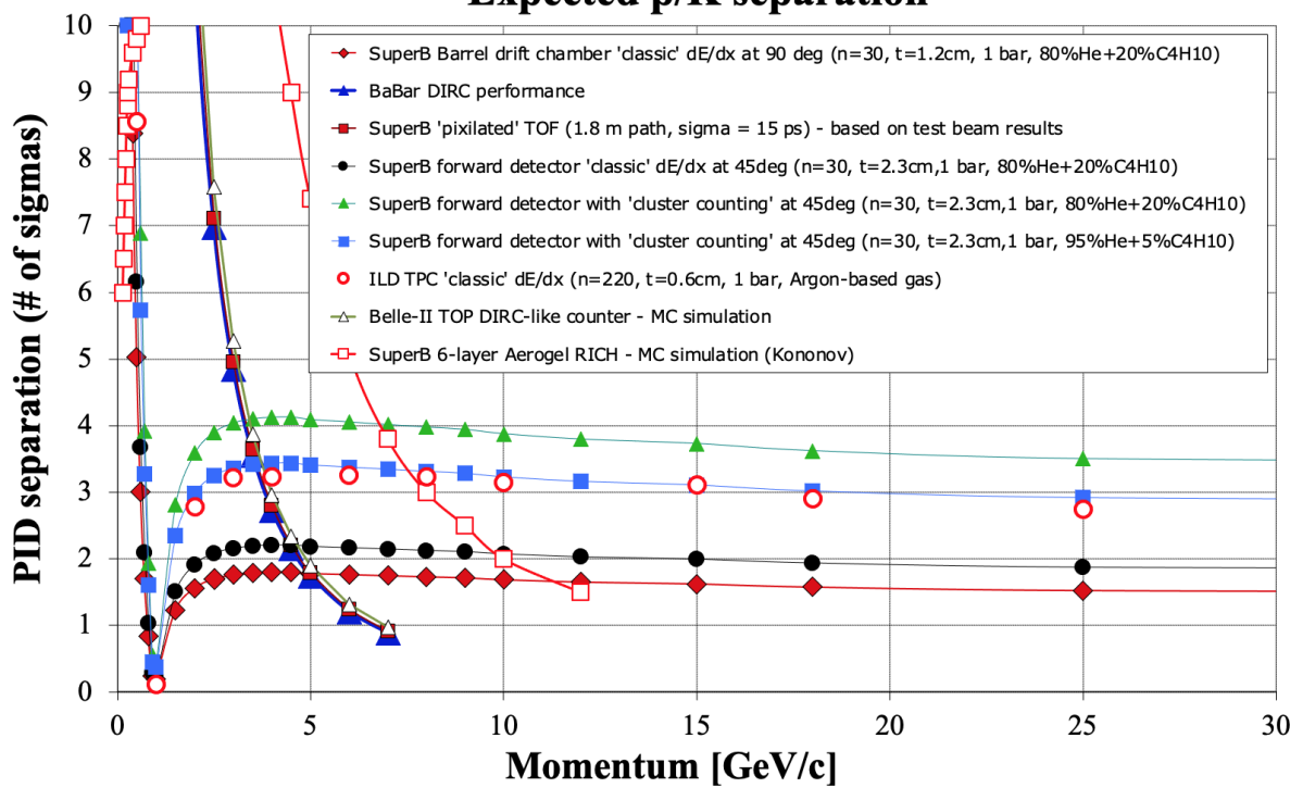
Figure E2: Expected \pi/K separation [98] reach in terms of number of sigma for TOF, dE/dx , BaBar DIRC, Belle-II TOP counter, aerogel detectors within SuperB [99] and Belle-II [100], and ILD TPC dE/dx MC simulation [41].
