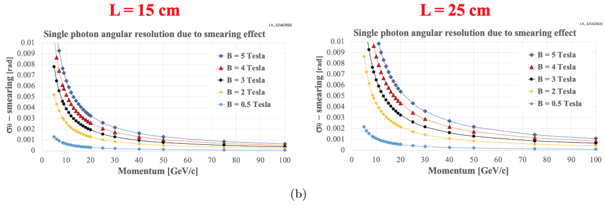
Figure 30: (a) Principle of the analytical calculation for the magnetic field smearing effect. (b) Angular resolution for two radiator lengths: L = 15 \text{ cm} and 25 \text{ cm} .
