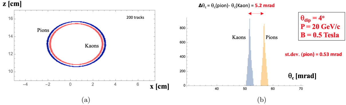
Figure 32: Smearing effect in the SLD CRID gaseous RICH for \theta_{\text{dip}} = 4^\circ , p = 20 \text{ GeV} , B = 0.5 \text{ T} , and L = 45 \text{ cm} . (a) Cherenkov rings imaged as 2D-hits, \{x_{\text{final}}[i], z_{\text{final}}[i]\} , in the SiPM detector plane with no cuts and no fitting, showing the smearing effect alone. (b) A plot of the Cherenkov angle \theta_c = (\text{Cherenkov radius}) / (\text{focal length}) , where the Cherenkov radius = \sqrt{(x_{\text{final}}[i] - x_0)^2 + (z_{\text{final}}[i] - z_0)^2} . We tune x_0 and z_0 to obtain the smallest possible standard deviation.
