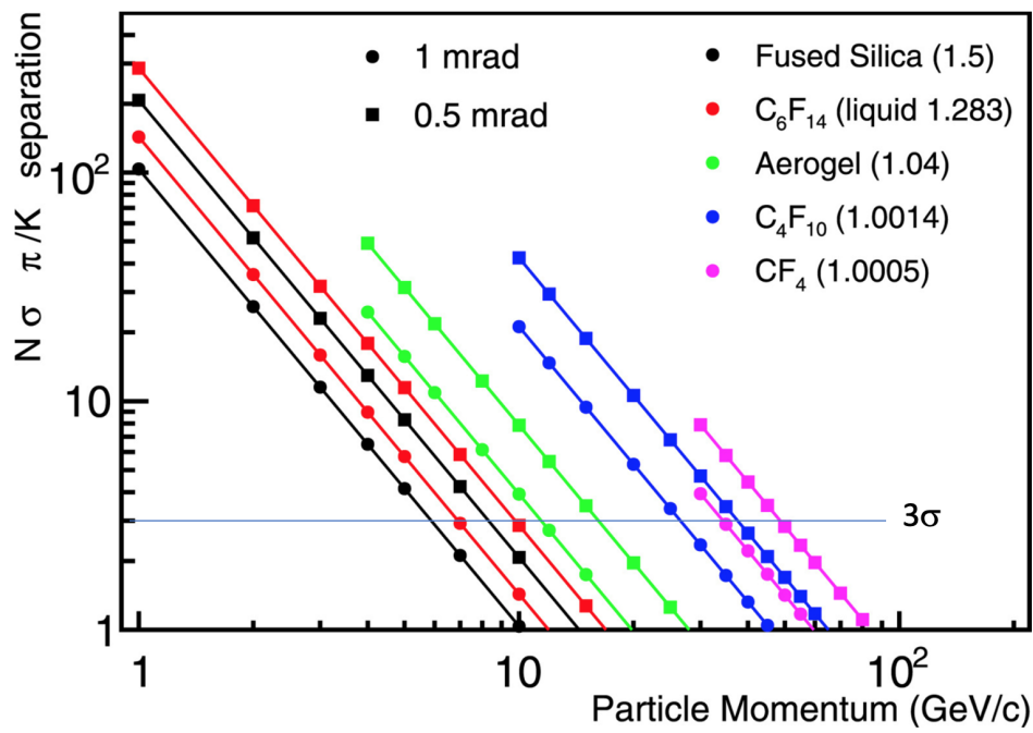
Figure E1: Expected \pi/K separation reach in terms of number of sigma for various radiator choices and for two Cherenkov angle resolutions, \sigma_{\text{tot}} = 0.5 and 1 mrad [96, 97]. In practice, the resolution tends to be worse when all contributions are included.
