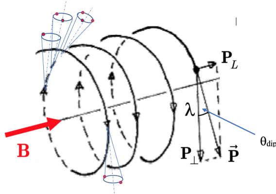
Figure 29: Schematic diagram of the helix trajectory and Cherenkov cones. Notice that the Cherenkov cones move in 3D. This contributes to smearing of the detected image at large magnetic field.
