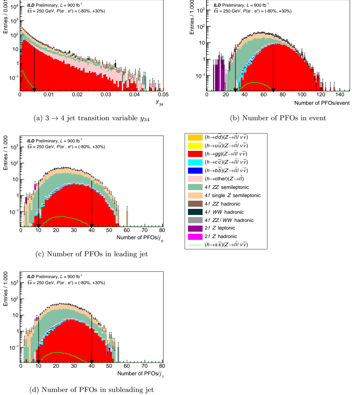
Figure 17: Histograms of the variables used in the kinematic selections of the Z \rightarrow \ell\bar{\ell} channel, as described in Table 3. Each histogram is given at the level of its corresponding selection but before that selection is applied. The arrows represent the placement of the selection cuts, and the error bars represent the MC statistical uncertainties. The sum-of-weights per process is normalised to the SM cross section. N.B. the h(\rightarrow s\bar{s})Z(\rightarrow \ell\bar{\ell}/\nu\bar{\nu}) signal is unstacked. A continuation of Fig. 16.
