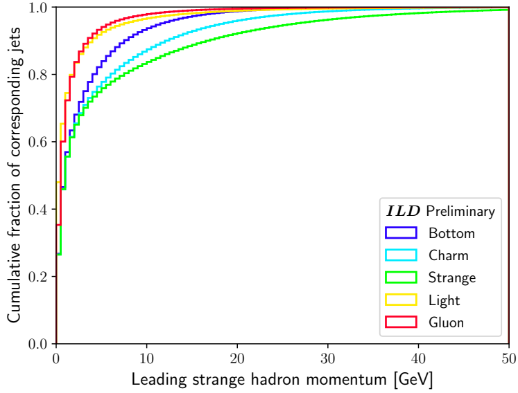
Figure 3: Differential and cumulative distributions of the momentum of the leading strange particle in the leading or subleading momentum jet of the h(\rightarrow q\bar{q}/gg)Z(\rightarrow \nu\bar{\nu}) events described in Table 2. The choice of leading or subleading jet is random. The leading strange particle is identified by iterating over the momentum-ordered PFOs in the jet and selecting the first PFO which is truth-matched to a strange hadron. If no strange particle is found, a momentum of 0 GeV is assigned. The sum-of-weights for each class is normalised to 1.
