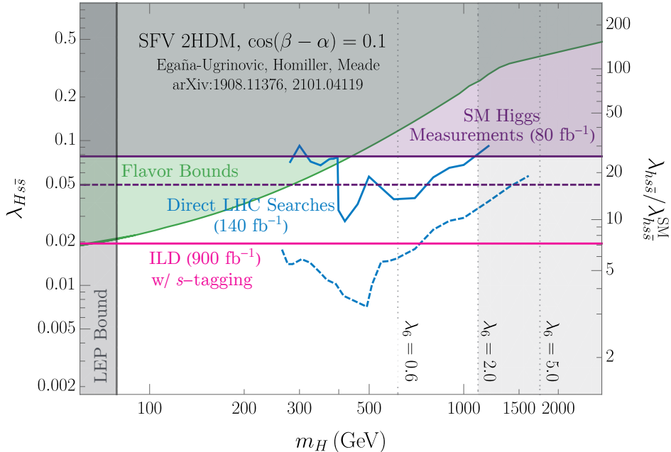
Figure 23: 95% CL bounds on the CP-even Higgs-strange Yukawa coupling \lambda_{Hs\bar{s}} as well as on 125 GeV SM Higgs-strange Yukawa coupling \lambda_{hs\bar{s}}/\lambda_{hs\bar{s}}^{\text{SM}} (i.e., \kappa_s ) for the SFV 2HDM described in Refs. [23, 24]. The limits are shown as a function of the mass of the CP-even Higgs, m_H . The model assumes the CP-even Higgs H , the CP-odd Higgs A , and the charged Higgs H^\pm are all degenerate (i.e., m_H = m_A = m_{H^\pm} ) – additionally, an alignment parameter of \cos(\beta - \alpha) = 0.1 is used for the h - H mixing. The green line shows the bounds obtained from D - \bar{D} mixing as described in Ref. [23]; the purple lines show the bounds obtained by requiring the inclusive gluon-gluon fusion cross section to be consistent with combination measurements from ATLAS [79]; the blue lines show the bounds obtained H \rightarrow hh and A \rightarrow Zh measurements from ATLAS and CMS [80, 81, 82]; and the pink line shows the bounds obtained from the h \rightarrow s\bar{s} analysis presented in this paper. The dashed lines correspond to bounds expected from the HL-LHC. Also shown are bounds from charged Higgs searches performed at LEP [83]. Drawn as dotted lines are the contours for the 2HDM’s quartic coupling \lambda_6 : \mathcal{L} \supset (\lambda_6 H_1^\dagger H_1 H_1^\dagger H_2 + \text{h.c.}) .
