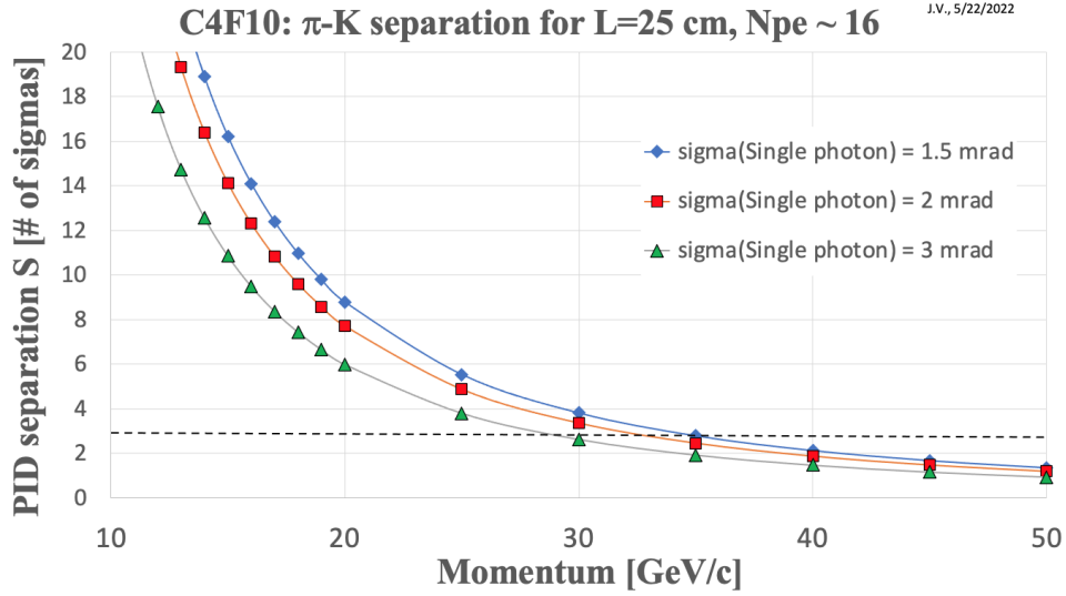
Figure 27: Expected PID performance as a function of momentum and (total) single-photon Cherenkov angle resolution. A resolution higher than 4mrad starts severely affecting the performance. Here, we assume 16 photoelectrons per ring and a tracking error of 0.5 mrad, which does not scale with N_{pe} .
