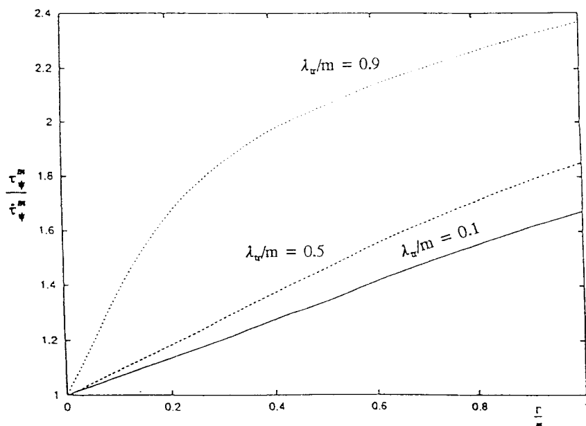
Fig. 3.2. The plot of \tau_\psi^m/\tau_\psi^m versus \Gamma/m for various \lambda_{tr} .
