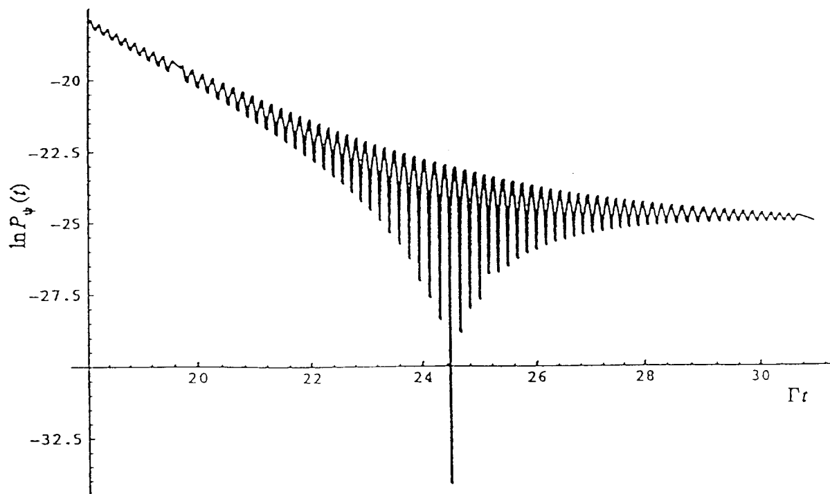
Fig. 2.4. The plot of \ln P_{\psi}(t) versus \Gamma t for Z^0 ( \lambda_r=0 ).
