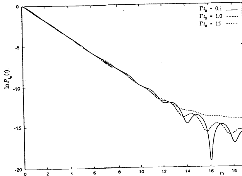
Fig. 3.3. The plot of \ln P_t(t) for various t_0 , \lambda_u/m = .1 and \gamma = .3
