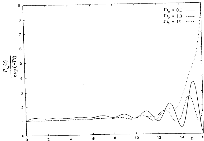
Fig. 3.4. The plot of P_t(t)/\exp(-\Gamma t) for the same parameters as in Fig. 3.3
