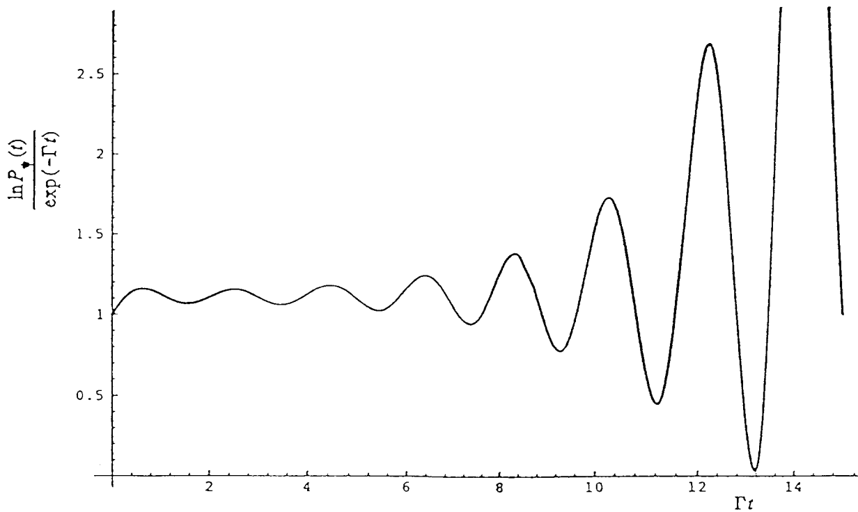
Fig. 2.2. The plot of P_\psi(t)/\exp(-\Gamma t) as the function of \Gamma t for \rho -meson
