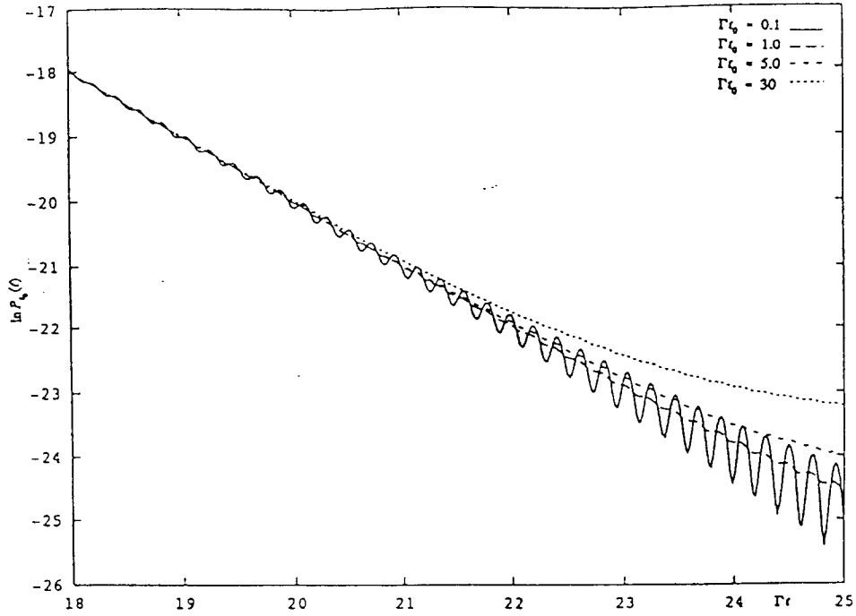
Fig. 3.5. The plot of \ln P_{t_0}(t) for various t_0 , \lambda_{tr}/m=.1 and \gamma=.03
