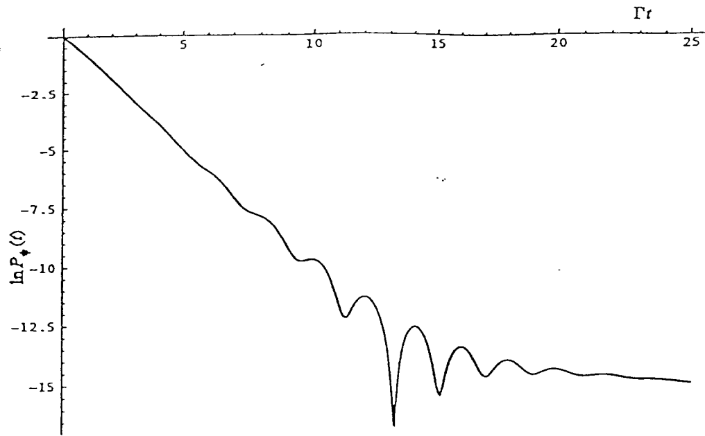
Fig. 2.1. The plot of \ln P_\psi(t) versus \Gamma t .
