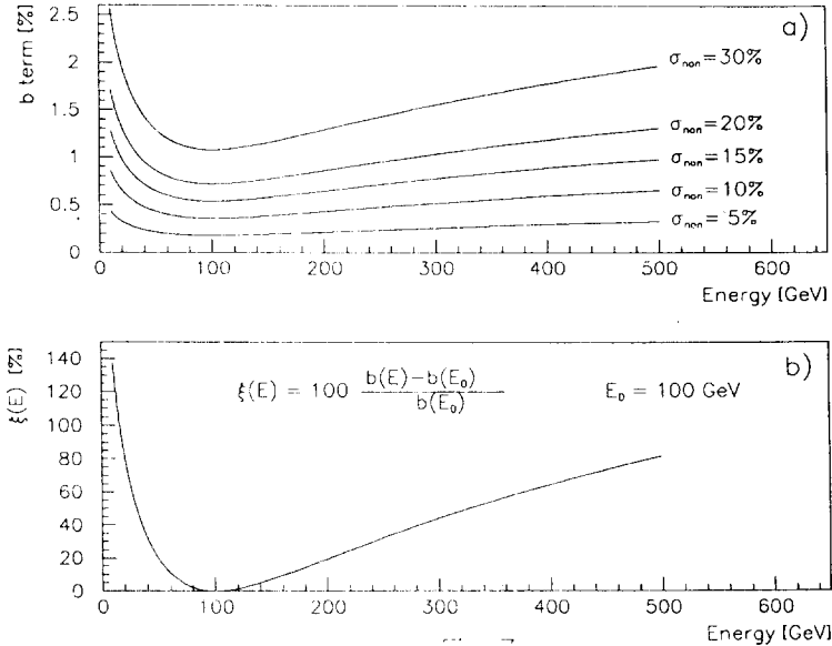
Fig. 7. (a) total contribution (i.e. b_0 \pm b_c^{tw} ) of tile nonuniformity to the b term for different \sigma_{\text{non}} , evaluated from results of the fit; (b) a measure of b variation over the whole energy interval, taking b(E_0) as a reference value.
