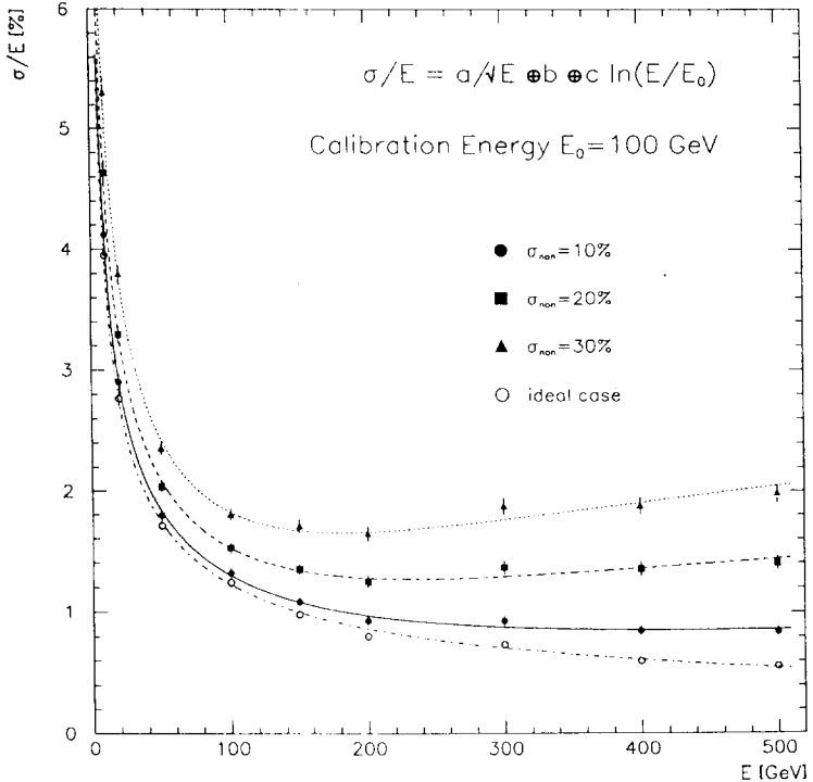
Fig. 5. Calorimeter energy resolution after tower by tower calibration, for different nonuniformities \sigma_{non} .
