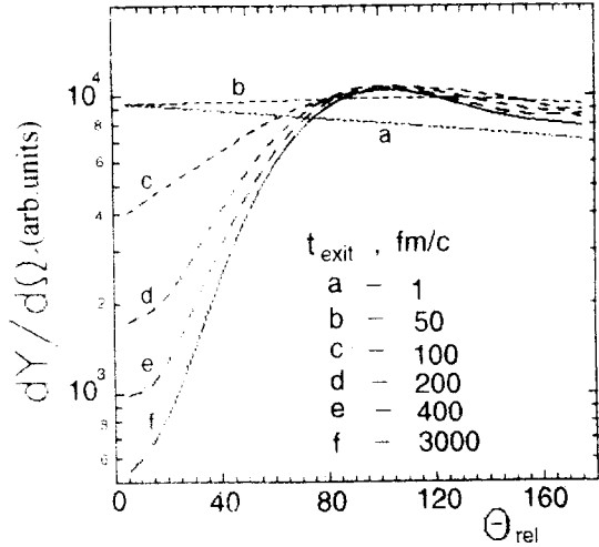
Fig. 1. Distributions of relative angles between coincident fragments at different times t_{\text{exit}} after the break-up moment.
