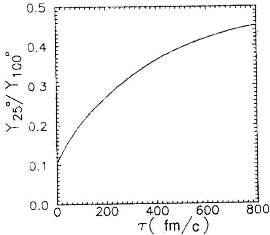
Fig. 3. The magnitude of the small relative angle suppression as a function of the mean lifetime of the fragmenting system.
