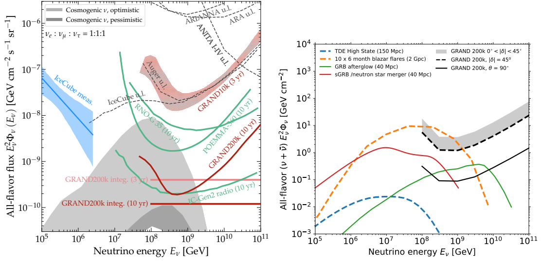
Figure 1: Left: Differential and integrated neutrino sensitivity limits calculated from the 10,000 antennas simulation ("GRAND10k", pink area) and the extrapolation for the 20-times larger GRAND array ("GRAND200k", maroon line). The gray region represents the all-flavor cosmogenic neutrinos flux expectations derived from the results of the Pierre Auger Observatory [5]. Adapted from [1]. Right: GRAND point source sensitivity limits [1]. Short-duration transients (short GRBs, GRB afterglows) are compared to the GRAND200k instantaneous sensitivity at zenith angle \theta = 90^\circ (solid black line). Long-duration transients (e.g., TDE) are compared to declination-averaged sensitivity (gray-shaded band). The stacked fluence from 10 six-month-long blazar flares in the declination range 40^\circ < |\delta| < 45^\circ is compared to the GRAND200k sensitivity for a fixed \delta = 45^\circ (dashed black line). The GRAND limits assume that the 200k antennas are deployed at a single location.
