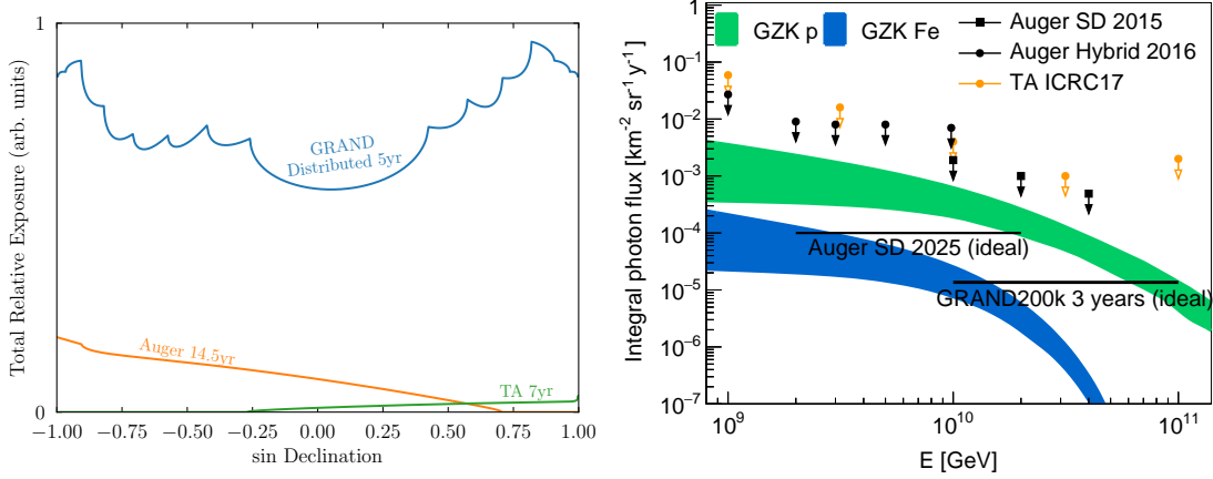
Figure 2: Left: The relative annual geometric exposure to UHECRs of GRAND for a uniform distribution of 10 sub-arrays on the Earth, compared to Auger and the Telescope Array (TA). Right: Projected upper limits of GRAND on UHE photon sensitivity after 3 years of operation. For comparison, we include the existing upper limits from Auger and TA, and the projected reach of Auger by 2025. Overlaid are the predicted cosmogenic UHE photon flux from pure-proton and pure-iron UHECRs, as estimated in [29].
