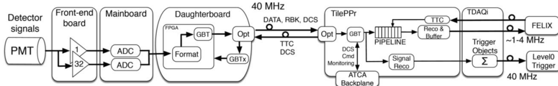
Fig.3. Block diagram of the HL-LHC readout architecture in TileCal.
