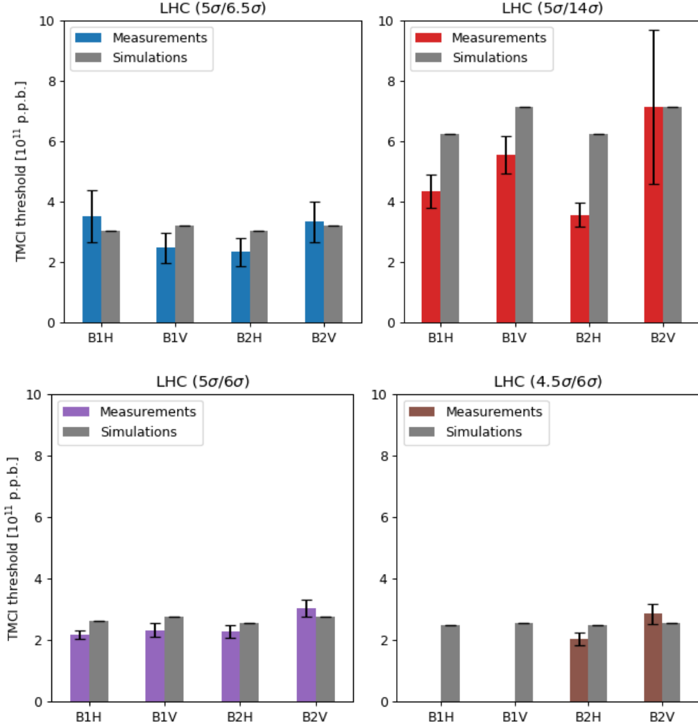
Figure 4: TMCI threshold extrapolated from the tune shift measurements for the operational ( 5\sigma_{coll}/6.5\sigma_{coll} ) and HL-LHC like ( 5\sigma_{coll}/14\sigma_{coll} ) scenarios (top) and for the tighter ( 5\sigma_{coll}/6\sigma_{coll} and 4.5\sigma_{coll}/6\sigma_{coll} ) collimator scenarios (bottom).
