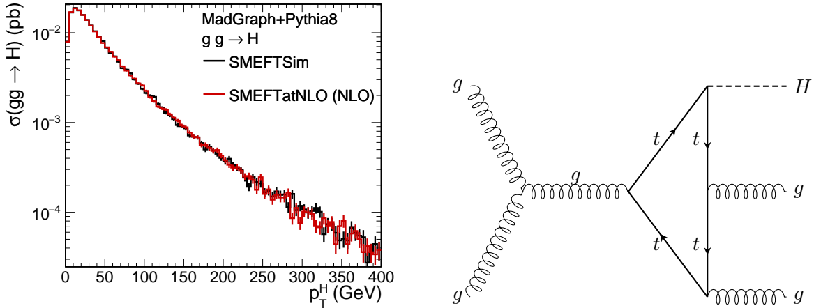
Fig. IV.16: Left: Comparison of the differential cross section of gg \rightarrow H as a function of p_T^H in SMEFTsim and SMEFT@NLO. Right: Example diagram contributing to gg \rightarrow H + j which is not considered in SMEFTsim but it is implemented in SMEFT@NLO.
