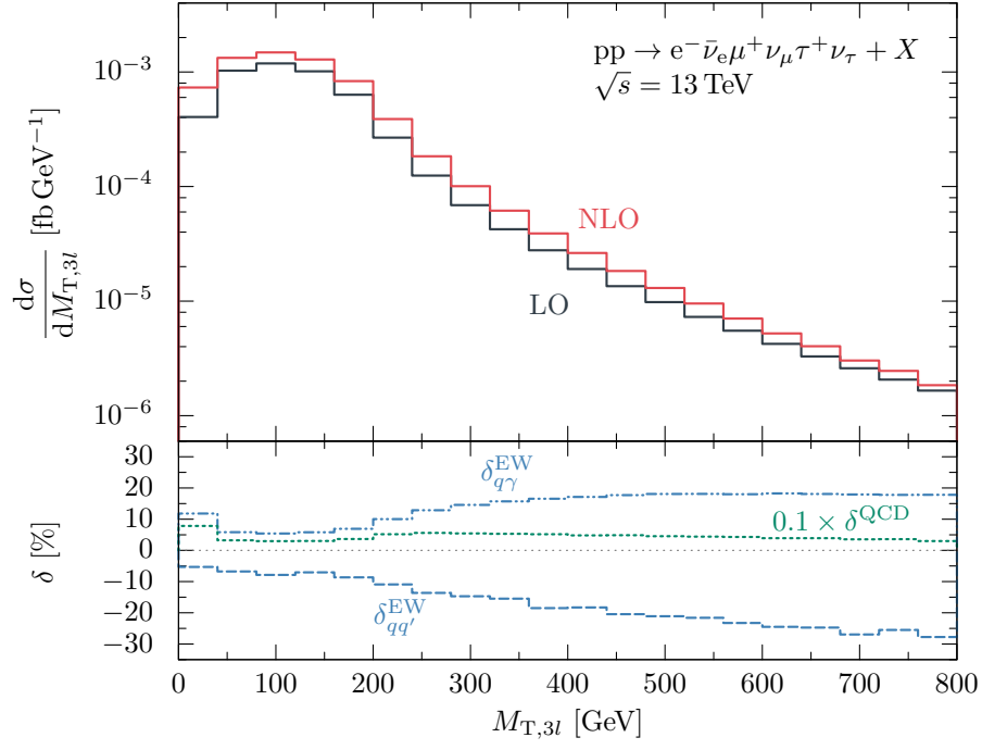
Fig. I.15: Differential distribution in the transverse mass M_{T,3\ell} of the three-lepton system. The NLO QCD correction \delta^{\text{QCD}} is scaled down by a factor of 10 for better readability.
