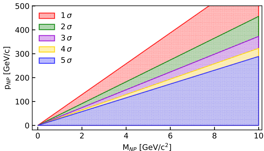
Figure 29: Sensitivity curves for a TOF measurement, illustrated from 1 up to 5\sigma in the plane (M_{\text{NP}}, p_{\text{NP}}) of the New Particle candidates to be detected in the SND@LHC detector, produced assuming a time resolution of \sim 200 ps.
