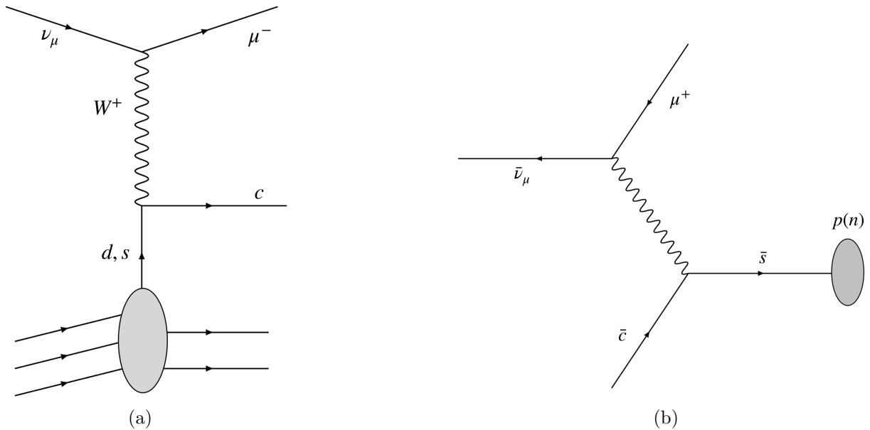
Figure 26: Charm production in neutrino (a) and anti-neutrino (b) charged-current interactions.
