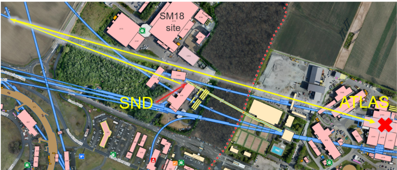
Figure 19: Preliminary optical fibres layout
