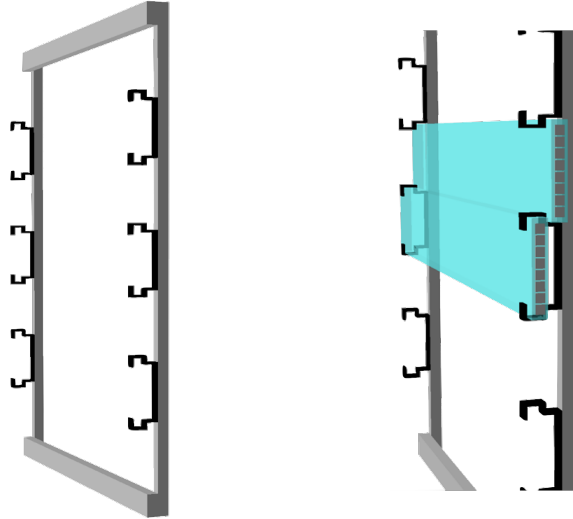
Figure 7: Left: Aluminium frame of the veto detector with plastic supports for the scintillating bars. Right: Illustration of how the scintillating bars will be supported on the aluminium frame. The location of the eight SiPMs on the end of the bars is also shown.
