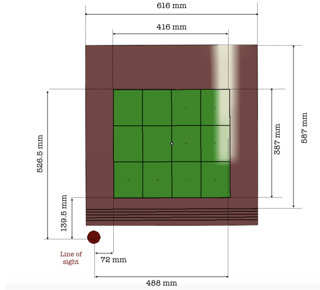
Figure 5: Frontal view of the detector.
