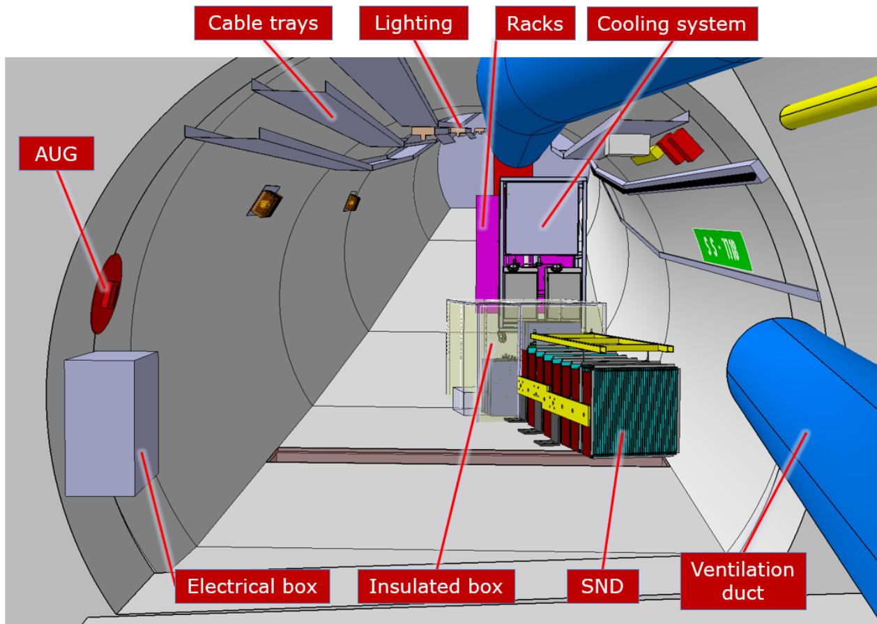
Figure 15: SND integration inside TI18
