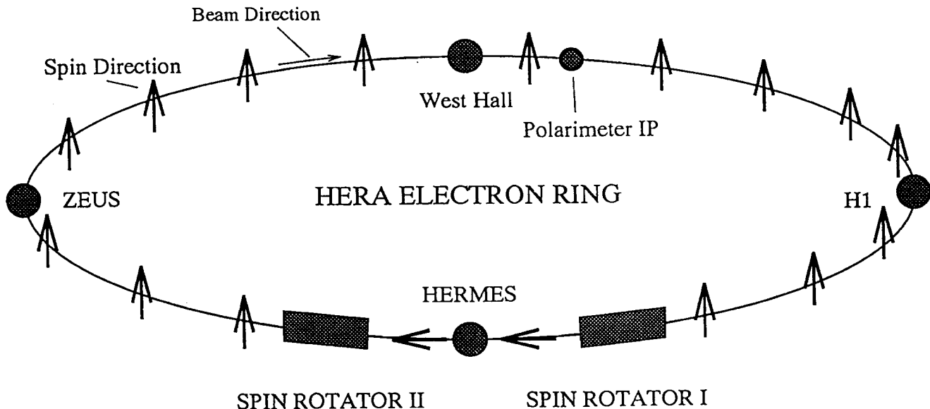
Figure 1: A sketch of the HERA electron ring showing the positions of the spin rotators and the polarimeter I.P. The directions of the momentum and the spin polarization of the electron beam are indicated; the current orientation of the spin direction at the East I.P. is parallel to the beam direction. The polarization is vertical at the position of the polarimeter I.P.
