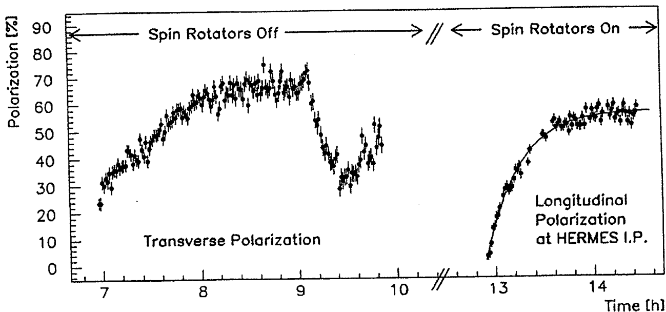
Figure 4: The polarization plotted as a function of time, measured on May 4, 1994. Shown are the measurements during the last fill with the spin rotators off, and the first fill with them on. The beam currents were initially 3 and 9 mA, respectively. The maximum polarization during the run before the rotators were switched on was 66.5 \pm 1.0\% . Between 10:00 and 12:45 the beam was dumped, the rotators switched on, and a new electron fill was injected and accelerated to 27.521 GeV. The polarization measured during this first fill is shown and the result of a fit of the expected exponential build-up curve to the data is overlaid. The results are P_{max} = 56.6 \pm 0.5\% and \tau = 20.8 \pm 0.7 minutes. The H1 solenoid and compensator were off during these measurements.
