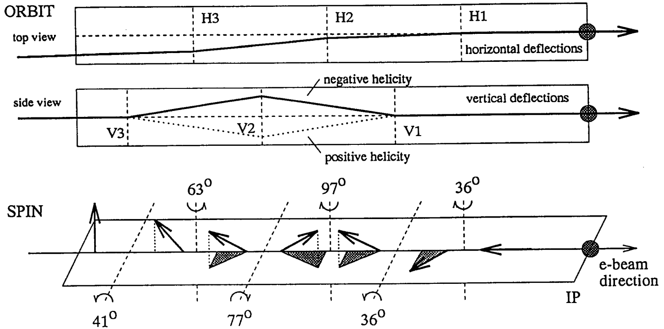
Figure 2: A functional diagram of the Mini-Rotator, showing schematically the horizontal and vertical orbit deflections produced by the dipole magnets and the corresponding spin precession angles. The rotation angles of the \hat{n}_0 axis correspond to a beam energy of 27.52 GeV. The net horizontal bend of the rotator is equal to that of two arc dipoles. The amplitude of the closed bump produced by the vertical deflections V_3 , V_2 and V_1 is approximately 20 cm. The two vertical bumps in a rotator pair are anti-symmetric, and to change the helicity of the polarization at an I.P. the directions of the bumps must be reversed; the dotted line indicates the bump geometry for the opposite helicity.
