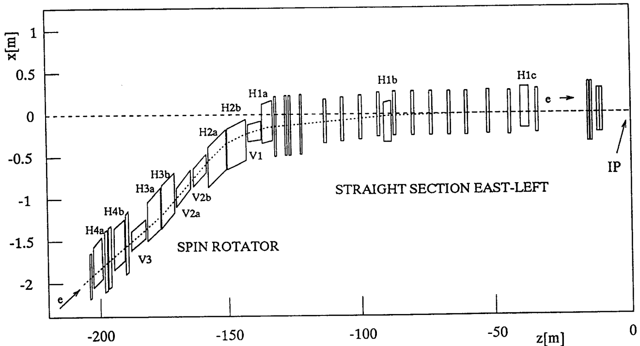
Figure 3: The layout of one 90^\circ Mini-Rotator as seen from above, showing the electron orbit and the magnet lattice in the straight section East-left. The dipole magnets (labeled, refer to fig. 2) and the quadrupoles are shown. The proton beam is offset by 71 cm at the East I.P. and is not shown. The foreseen layout of the rotators for the North and South areas, where the beams collide, is somewhat different. The horizontal deflection H1 is split, with H1-a chosen to be a relatively weak dipole, in order to reduce the synchrotron radiation background at the HERMES interaction region; the dipoles H1-a and H1-b provide a rotation of the spins of 11^\circ . The magnets H4-a and H4-b are not utilized for the spin rotation but for the adjustment of the net horizontal orbit deflection in the rotator. As discussed in section 3, the actual spin match for HERA with one pair of rotators is achieved by obtaining spin transparency across the I.P. between magnets V2-b on the left and V2-b on the right; and separately, around the remainder of the ring.
