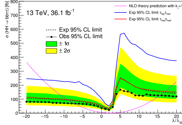
Figure 7.6: Expected and observed bb\tau\tau combined upper limits on the non-resonant di-Higgs production cross section times bb\tau\tau BR as a function of k_\lambda . The yellow and green bands represent the \pm 2\sigma and \pm 1\sigma variations about the expected limit. Expected limits from the single channels are also overlaid, in blue for the \tau_{lep}\tau_{had} channel and red for the \tau_{had}\tau_{had} one. The theoretical prediction of the cross section as a function of k_\lambda with k_t = 1 is also shown.
