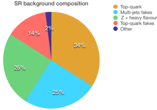
Figure 6.6: Background composition of the signal region.
