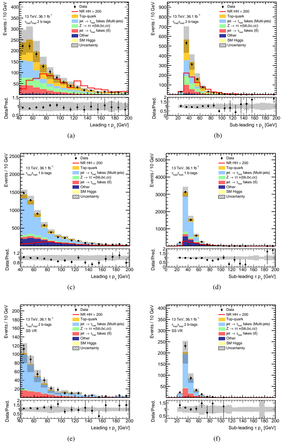
Figure 6.7: Data/prediction comparison in the distributions of the leading and sub-leading \tau_{had-vis} p_T in the a), b) signal region, c), d) 1 b -tag and e), d) 2 b -tags SS validation regions. The uncertainty band includes both statistical and systematic uncertainties.
