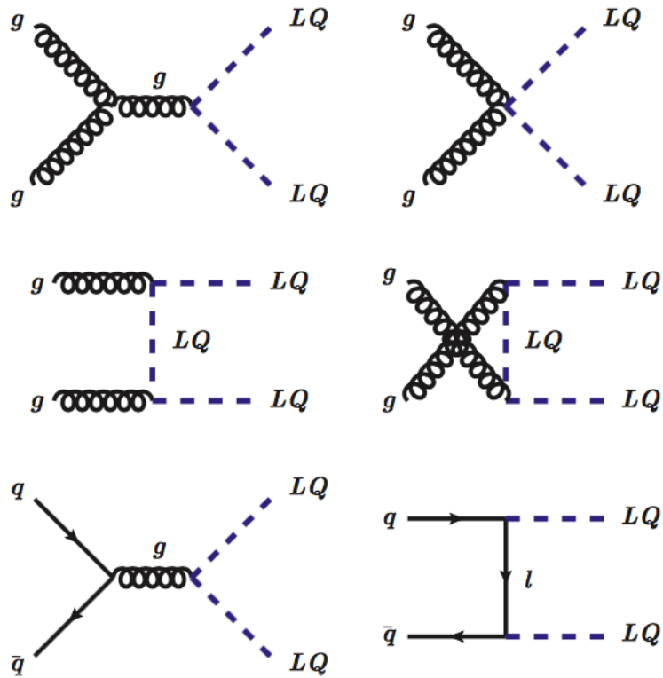
Figure 3.3: Leading Order Feynman diagrams of LQ pair production.
