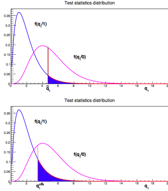
Figure 6.16: Construction of the CL_{s+b}^{exp} (upper plot) and CL_{s+b}^{obs} (lower plot). In both cases the CL_{s+b} is given by the blue area.
