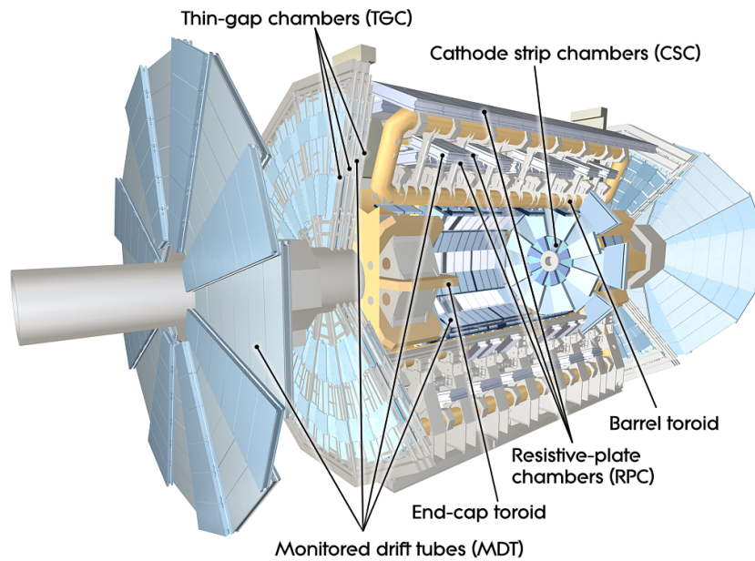
Figure 4.12: View of the ATLAS muon spectrometer [82].
