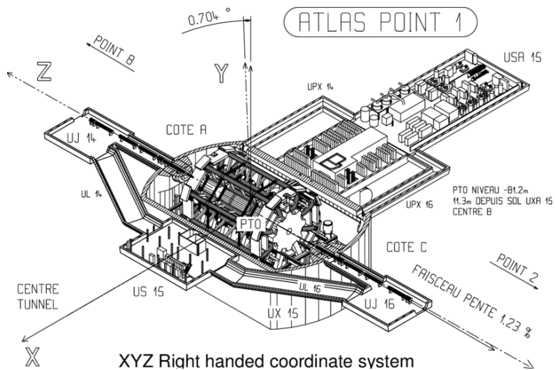
Figure 4.8: The coordinate system of the ATLAS detector [52].
