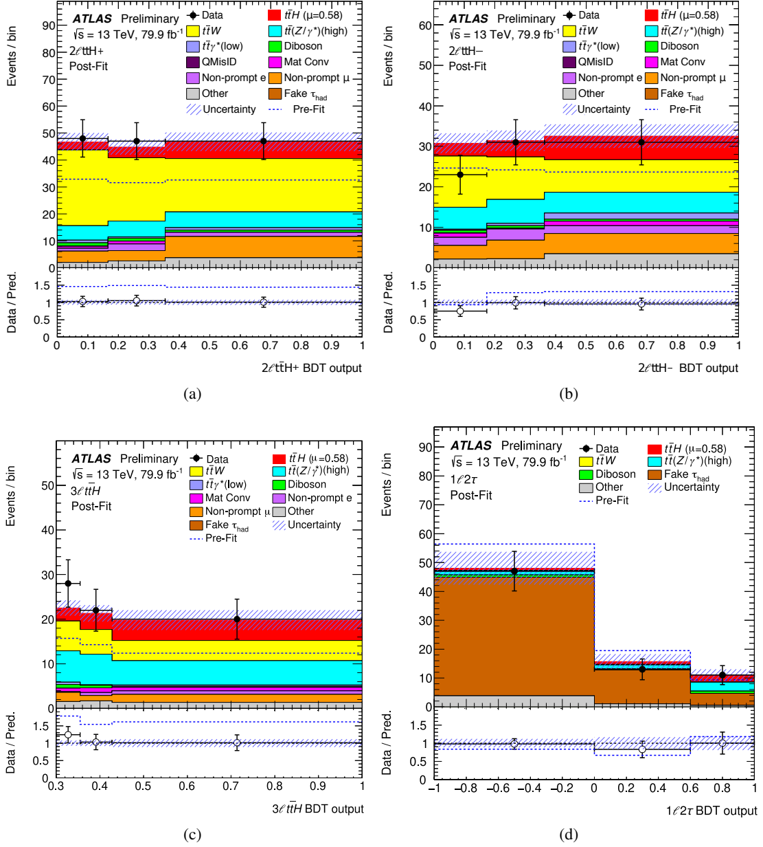
Figure 6: Comparison between data and prediction for the BDT discriminants used in different t\bar{t}H categories: (a) 2\ell ttH+ , (b) 2\ell ttH- , (c) 3\ell ttH , and (d) 1\ell 2\tau_{had} . The background contributions after the likelihood fit (“Post-Fit”) are shown as filled histograms. The total background before the fit (“Pre-Fit”) is shown as a dashed blue histogram. The t\bar{t}H signal, scaled according to the results of the fit, is shown as a filled red histogram added to the post-fit background. The size of the combined statistical and systematic uncertainty in the total signal-plus-background prediction is indicated by the blue hatched band. The ratio of the data to the total post-fit prediction is shown in the lower panel.
