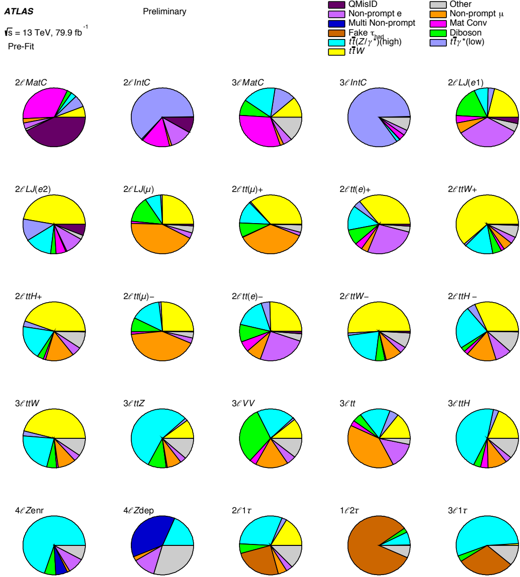
Figure 10: The fractional contributions of the various backgrounds to the total predicted background in each of the 25 event categories. The background estimation methods are described in Sect. 6: “Non-prompt ( e/\mu )”, “Mat Conv”, and “QMisID” refer to the data-driven background estimates (largely t\bar{t} but also include other electroweak processes), and rare processes ( tZ , tW , WtZ , t\bar{t}WW , VVV , t\bar{t}t , t\bar{t}t\bar{t} , and tH ) are labelled as “Other”.
