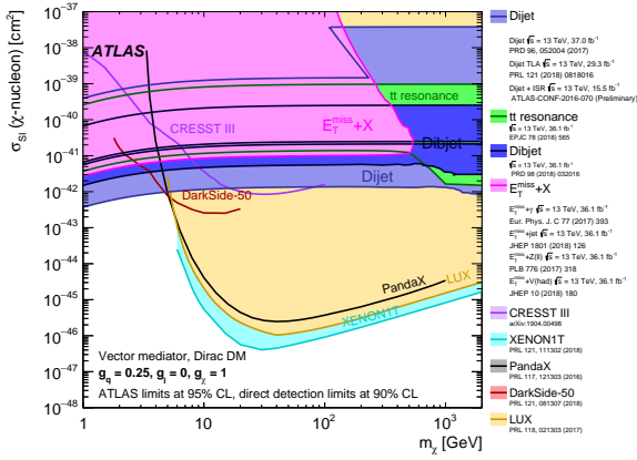
(a) Limits on the spin-independent WIMP–nucleon scattering cross section for a Z' vector mediator model.
