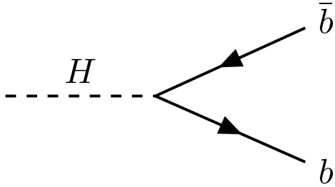
(a) Feynman diagram for Higgs decay to b\bar{b} .
