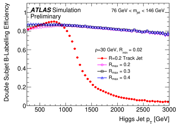
(c) The efficiency for VR track jets with \rho = 30 GeV and R_{\min} = 0.02 for varying values of R_{\max} .
