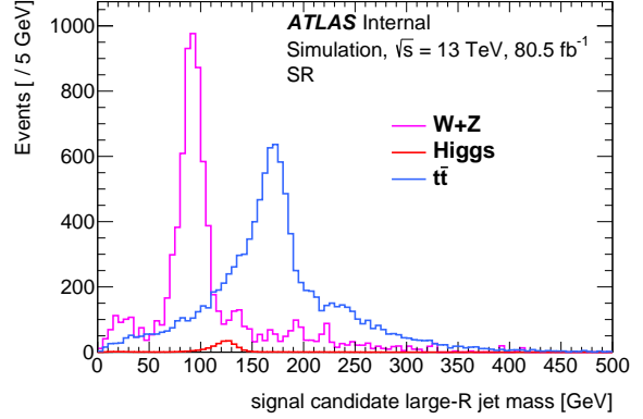
(b) Simulation of the resonant V + \text{jets} and t\bar{t} backgrounds in the signal region. Simulation of the Higgs boson signal is shown for comparison.
