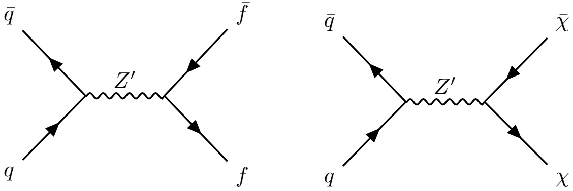
(a) Feynman diagram of the interactions of the Z' mediator with Standard Model fermions.
