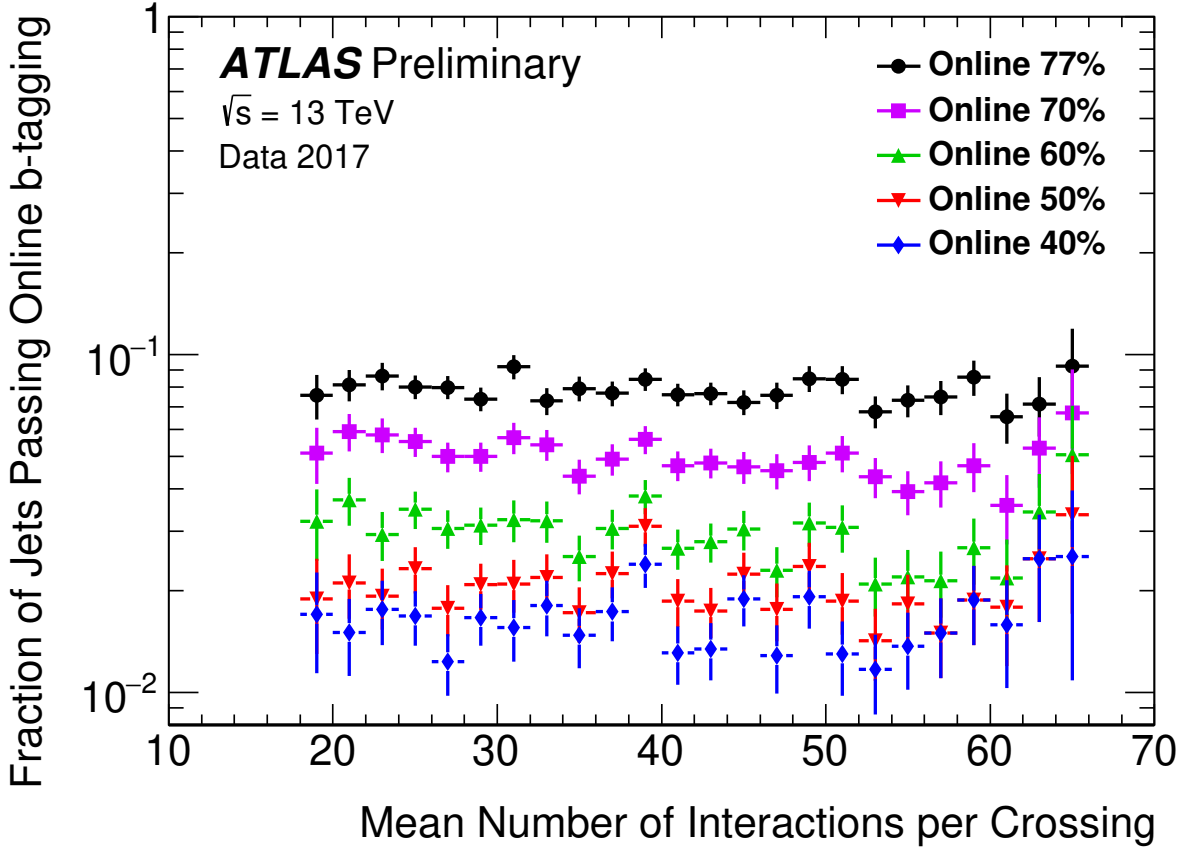
Figure 1.3: The fraction of trigger jets with Global Sequential Calibration (GSC)-corrected E_T > 55 GeV that pass the online b -tagging algorithm (MV2c10) at various online efficiency operating points vs. the mean number of interactions per crossing. The pass fraction is measured in a subset of the 2017 data-set with events containing at least one jet with GSC-corrected E_T > 55 GeV. The trigger used is unbiased with respect to the online b -tagging. The online operating points were defined to have roughly the quoted efficiency for b -jets in an unbiased sample of Monte Carlo simulated t\bar{t} events. The uncertainty bars shown only represent statistical uncertainties [188].
