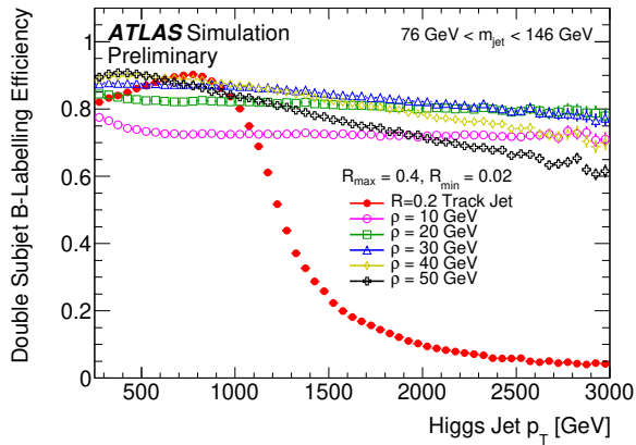
(a) The efficiency for VR track jets with R_{\min} = 0.02 and R_{\max} = 0.4 for several \rho values.
