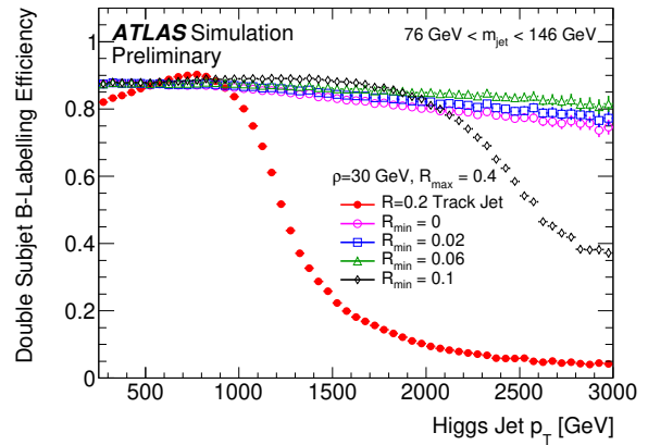
(b) The efficiency for VR track jets with \rho = 30 GeV and R_{\max} = 0.4 for different values of R_{\min} .
