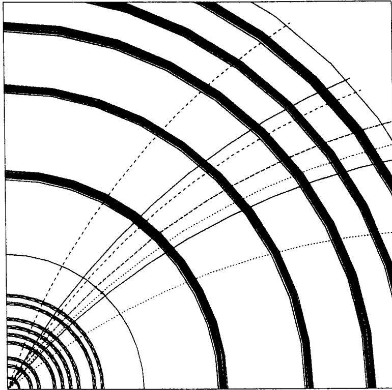
Figure 10: End view of a low P_t track passing through the overlapping zones used in the zonal track finding method. Solid, dashed, and dotted zone outlines are used to help distinguish between overlapping zones.
