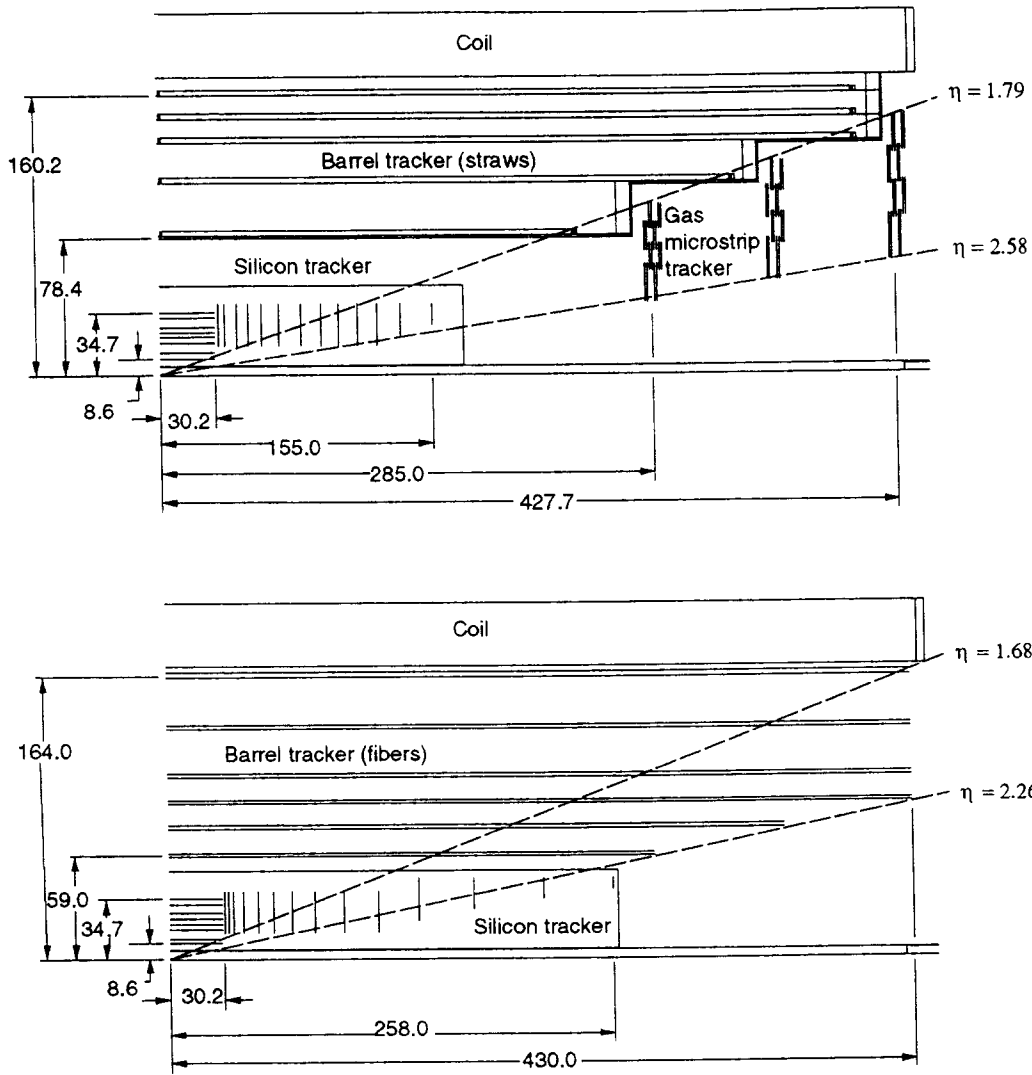
Figure 1: (a) SDC baseline charged particle tracking system; (b) tracking system with scintillating fiber outer tracker.
