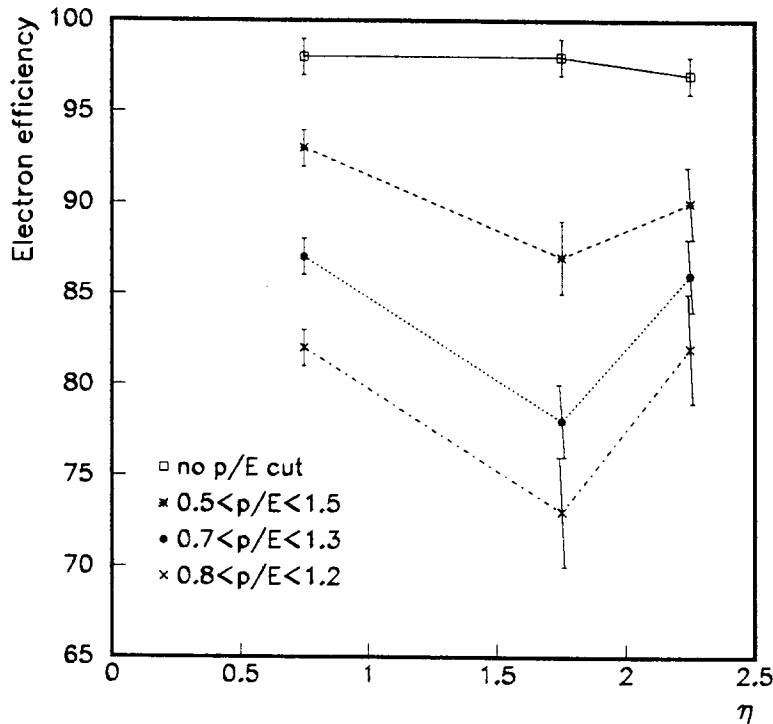
Figure 20: Track finding efficiencies for Higgs electrons for p/E > .8 , p/E > .7 , p/E > .5 and no p/E cut.
