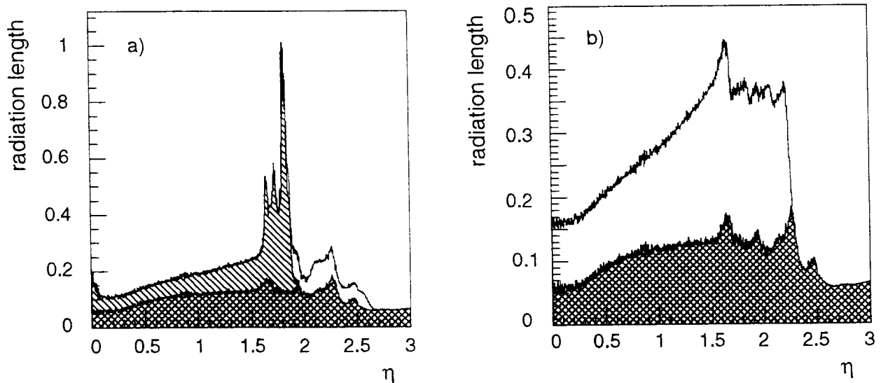
Figure 7: Material in the tracking system as a function of pseudorapidity for (a) the straw/ITD version, and (b) the scintillating fiber version. The double hatching corresponds to the silicon tracker, the single hatching represents the straw tubes in (a) and the scintillating fibers in (b), and the unhatched region in (a) represents the gas microstrip tracker.
