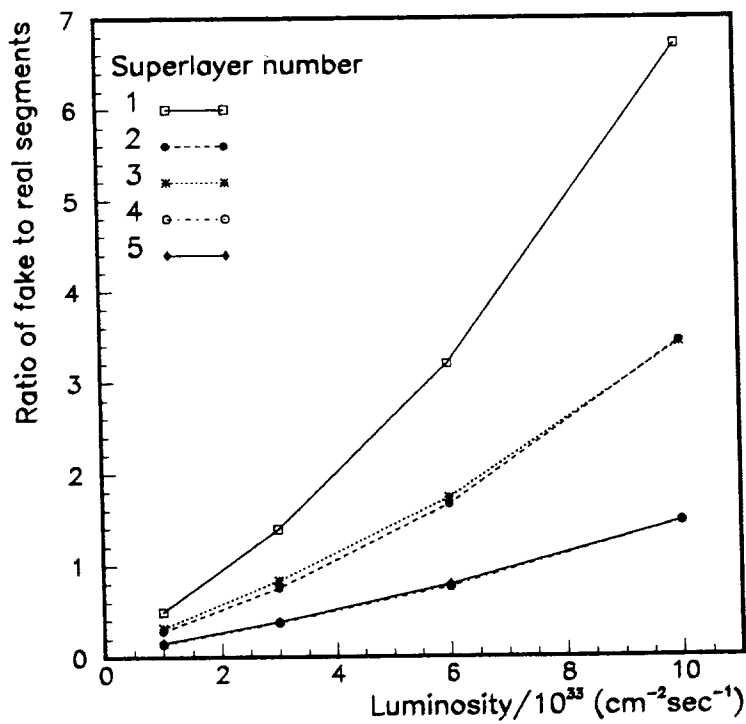
Figure 14: Ratio of fake to real segments vs luminosity for each superlayer of the straw tracker.
