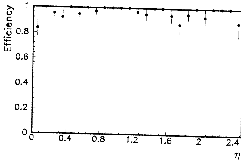
Figure 15: Track finding efficiencies as a function of pseudorapidity for Higgs muons at L=3 \times 10^{33} \text{ cm}^{-2} \text{ sec}^{-1} .
