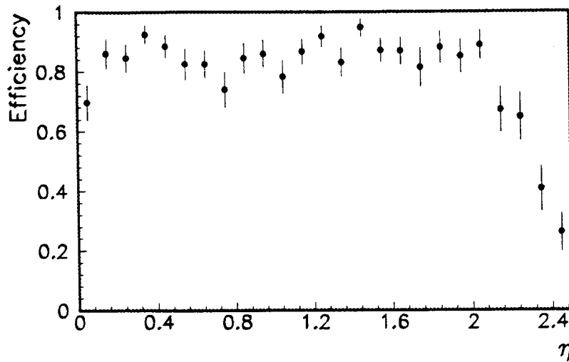
Figure 23: Track finding efficiencies as a function of \eta for all tracks with p_t > 1 GeV/c in a descoped silicon tracker.
