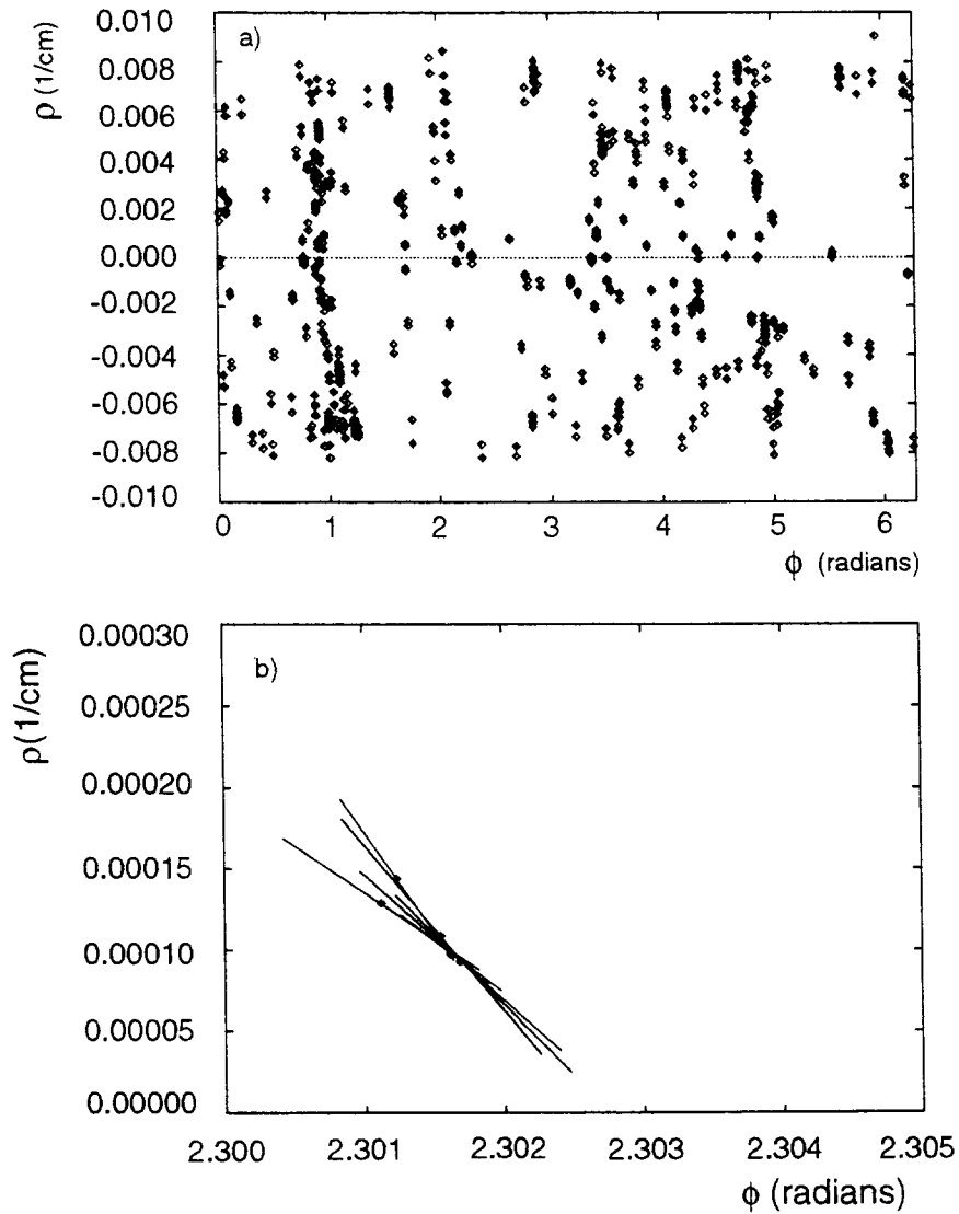
Figure 9: Distribution of barrel silicon segments in the (\phi_0, \rho) plane from a single Higgs event: (a) whole event; (b) single track.
