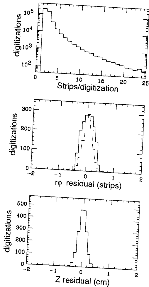
Figure 3: (a) Number of silicon strips in cluster; (b) fitted track residuals in r\phi for clusters in the barrel silicon detector. The solid (dashed) histogram is for single (double) strip clusters; (c) z residuals in the barrel silicon detector.
