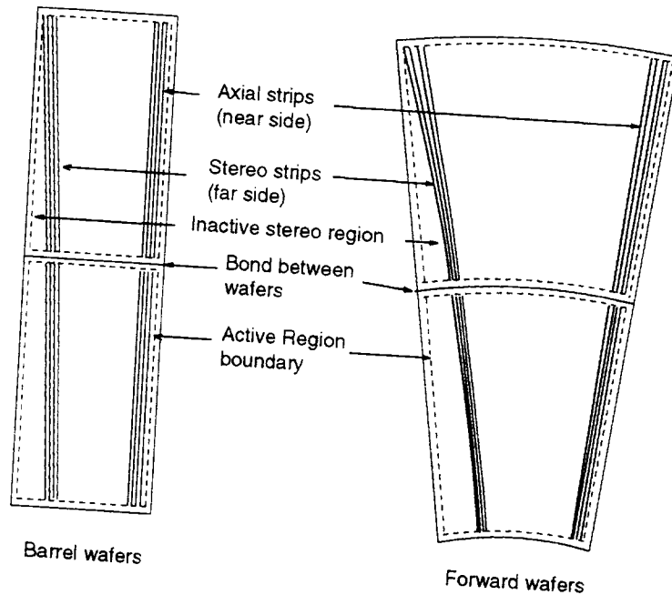
Figure 2: Barrel and forward wafers of silicon microstrip system.
