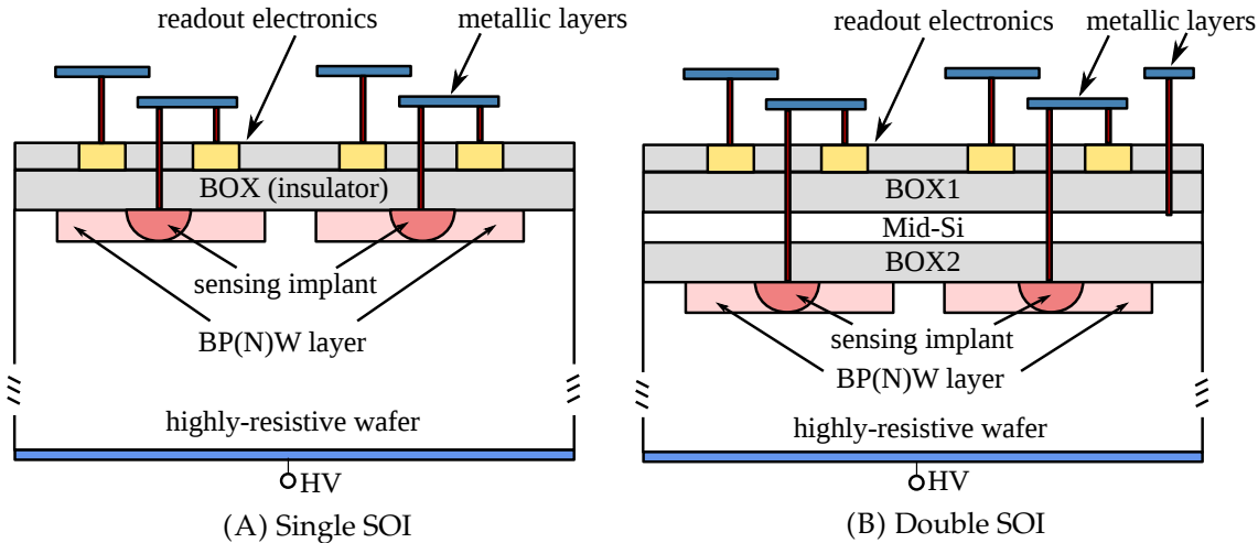
FIGURE 1.9: SOI detector schemes [32].
