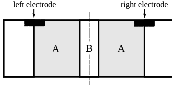
FIGURE 4.8: Sketch of two-electrode detector with definition of A region with no charge sharing and B with charge division [53]. Electric field forces charges on each side of the border to drift towards the closest electrode.
