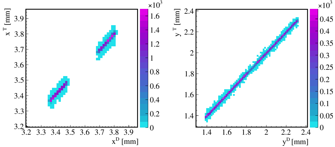
FIGURE 4.13: Track-hit positions correlation for x (left) and y (right) coordinate. Example shown for the FZ-n wafer. The gap in x is coming from physical gap between charge preamplifiers and source followers matrices.
