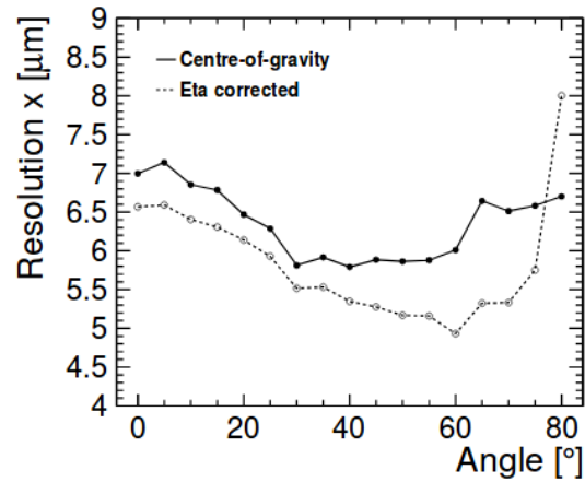
(B) Single-hit resolution at different angles [27]
