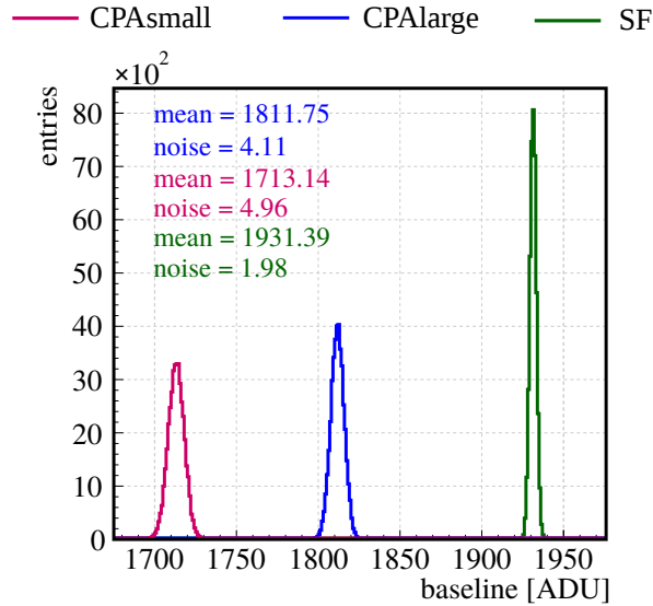
FIGURE 4.3: Single pixels baseline spectra for different matrices. The mean value of a spectrum is taken as a pixel baseline and its standard deviation as noise.
