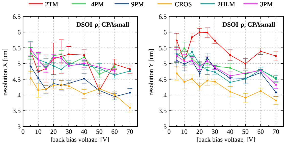
FIGURE 5.29: Final spatial resolution \sigma_{\text{res}} for CPAsmall on the DSOI-p wafer in function of back bias voltage for different clusterization methods.
