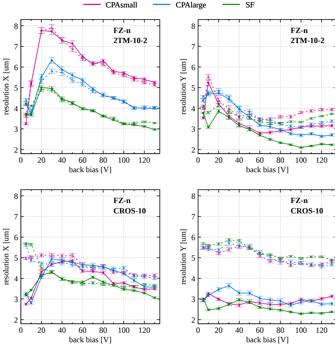
FIGURE 5.26: Comparison of final spatial resolution \sigma_{\text{res}} using 2TM-10-2 and CROS-10 for COG (dashed) and mp- \eta corrected positions (solid) for the FZ-n.
