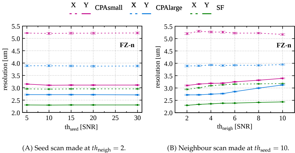
FIGURE 5.23: Final spatial resolution \sigma_{res} scan over thresholds in 2TM. Relations shown for the FZ-n wafer at 130 V.
