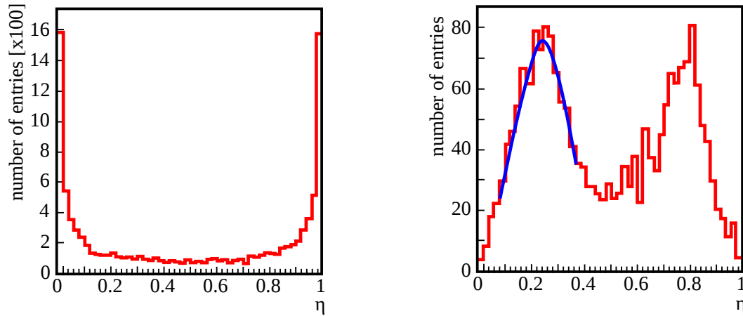
(A) Monte Carlo simulation in the absence of noise and capacitive coupling. (B) Experimental distribution for 50 \mu\text{m} strip detector and SNR = 10.
