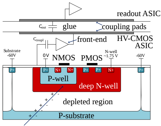
(A) HV-CMOS as a particle detector [28]
