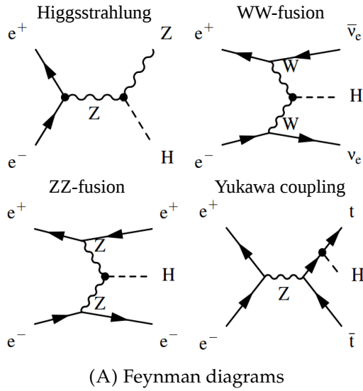
FIGURE 1.2: Main processes of Higgs production at CLIC [10]. The values for cross-sections (1.2B) shown for unpolarized beams and do not include the effect of the Beamstrahlung.
