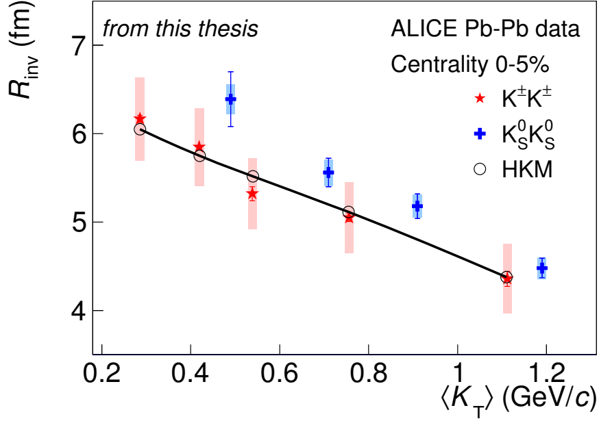
Figure 7.9: Comparison of the HKM model predictions for R_{\text{inv}} with the ALICE neutral and charged kaon results. The model predictions shown here are for K^\pm K^\pm . Statistical (thin lines) and systematic errors (rectangles) are shown.
