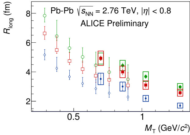
Figure 7.14: 3D LCMS radii vs. M_T for K_S^0 K_S^0 and \pi\pi from ALICE. For the kaons, statistical (thin lines) and systematic (boxes) errors are shown. For the pions, systematic errors (thin lines) are shown, while statistical errors are negligible. The pion points are averaged from narrower centrality bins (as told in the legend). The systematic errors for the pions are the maximum errors from the pre-averaged points.
