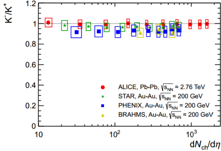
Figure 5.2: K^-/K^+ asymmetry results from ALICE [23], suggesting the lack of K^0/\bar{K}^0 asymmetry.
