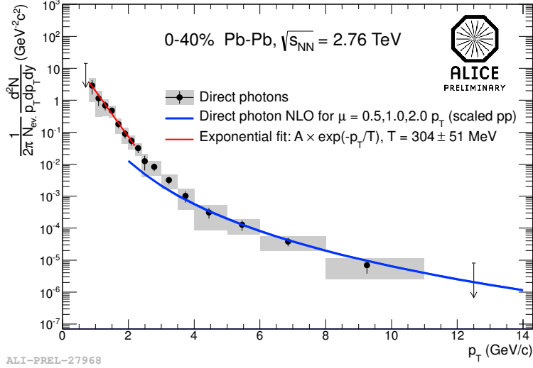
Figure 2.8: Direct photon invariant yield measured by ALICE in Pb-Pb collisions at \sqrt{s_{\text{NN}}} = 2.76 TeV for 0-40% centrality. Note the excess of photons at low p_T over the NLO predictions from scaled pp collisions, suggesting a thermalized medium, i.e. QGP. The low- p_T distribution is fit with an exponential to extract an effective temperature.
