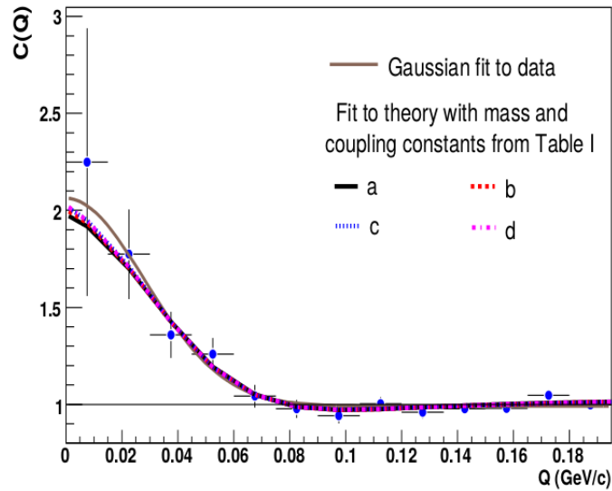
Figure 5.8: K_S^0 K_S^0 correlation function from the STAR experiment [148]. The different fits refer to different sets of FSI parameters, similar to Fig. 5.6 of this thesis.
