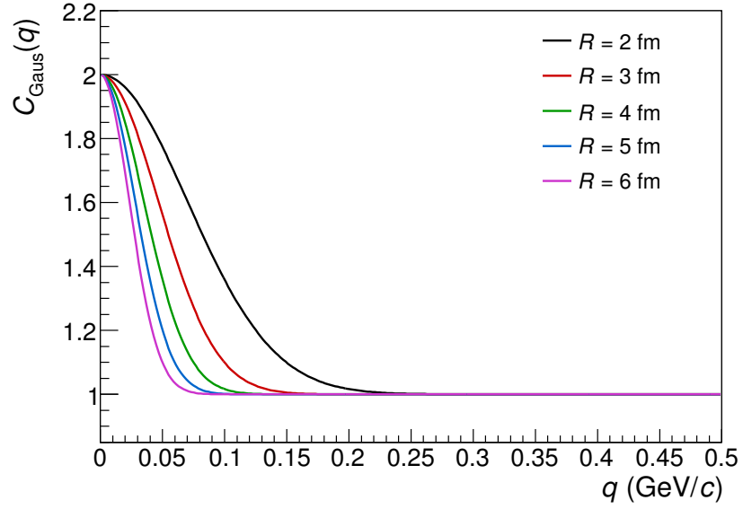
Figure 5.3: Bose-Einstein contribution to the K_S^0 K_S^0 correlation function for various radii.
