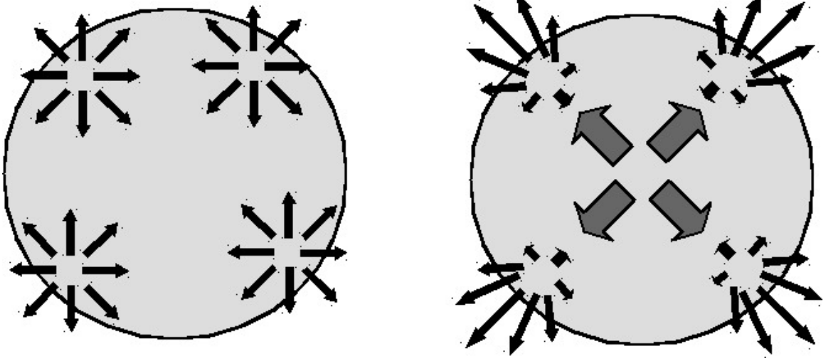
Figure 4.2: View of particle emission in transverse plane. Black arrows represent particle momentum. (Left) Thermal emission 8 from a static source. The region of particles with similar momenta approaches the full source size. (Right) Emission from an expanding source, with collective flow (represented by gray arrows) added to thermal emission. It is still possible for pairs with similar momenta at low pair momentum K_T to be emitted from different sides of the source; however, pairs with large K_T will only be emitted from the same side of the source.
