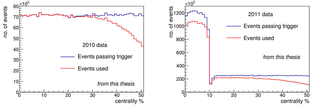
Figure 6.2: The centrality distributions measured from ALICE data from 2010 (left) and 2011 (right). The blue line refers to the events that passed the trigger and off-line physics selection, and the red line shows the events that were used in the analysis (passing z -vertex cut and possessing two K_S^0 particles).
