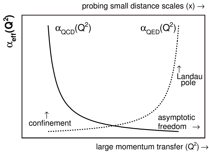
Figure 2.4: Qualitative diagram of the running coupling parameters for QCD and QED, showing the opposite trends exhibited by the two forces [5].
