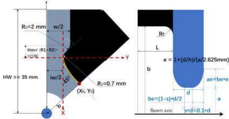
Figure 6. Sketch of a single cell geometry.
