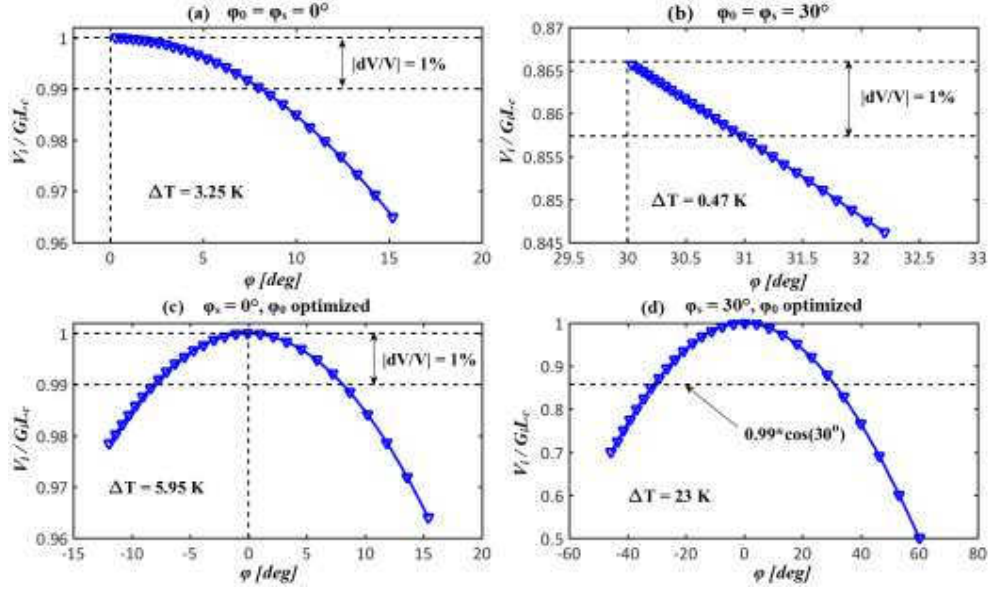
Figure 5. The distributions of the RF phase and accelerating voltage error in each cell caused by systematic temperature errors in the unloaded case for the four different conditions in CLIC-K. Table 2. Tolerances on systematic temperature errors given by accelerating voltage error limited to < 1% and < 2% in CLIC-K.
