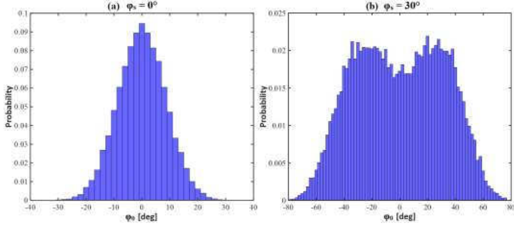
Figure 13. The distributions of optimized RF input phase \varphi_0 for two different synchronous phase in loaded case of CLIC-K.
