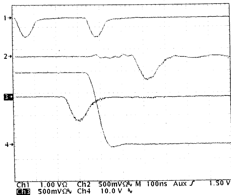
Figure 5. Oscilloscope traces showing the action of the E-field kicker on the double pulse of muons
