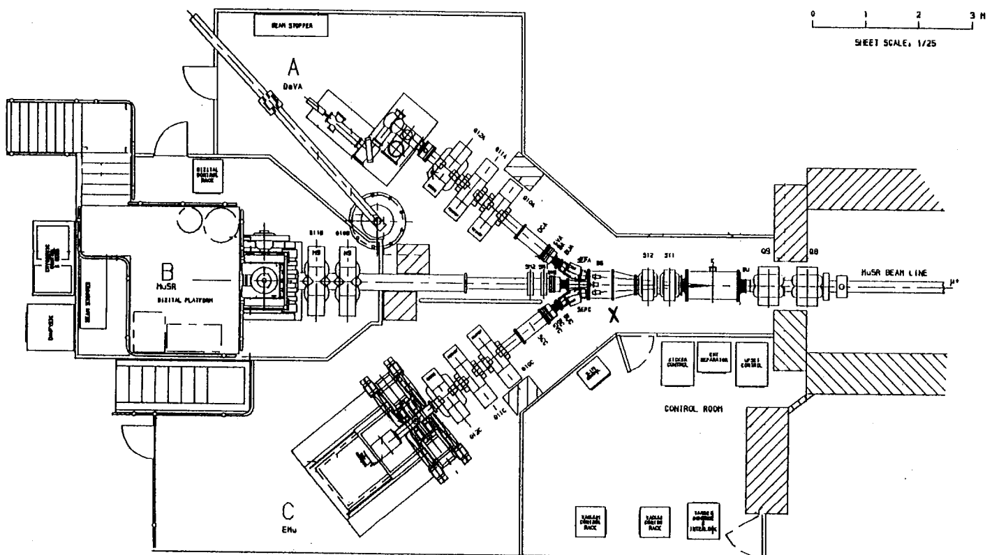
Figure 6. Layout of ISIS Pulsed Muon Facility
