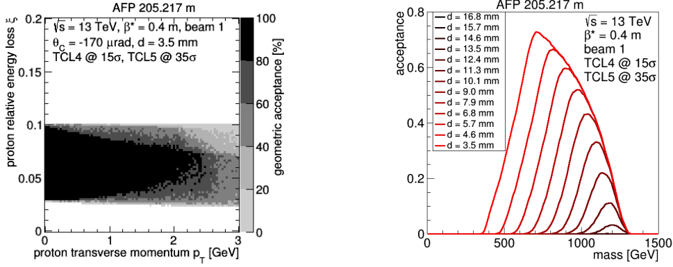
Figure 5: Near station acceptance: geometric (left) and mass (right). From [4].
