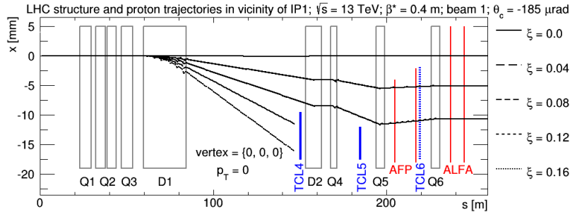
Figure 3: Proton trajectories between the ATLAS interaction point and the AFP detectors, from [6].
