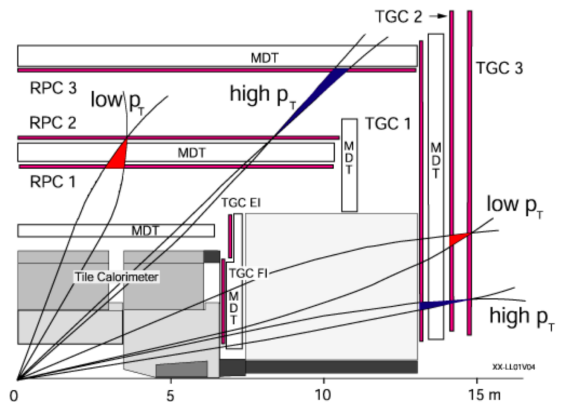
Fig. 2. The low- p_T and high- p_T trigger scheme, with the middle-pivot (RPC2), the inner low- p_T (RPC1) and the outer high- p_T (RPC3) detector. [4]
