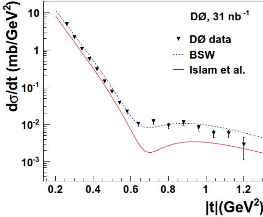
Figure 1: The measured differential elastic cross section from the D0 experiment at the Tevatron [3]
