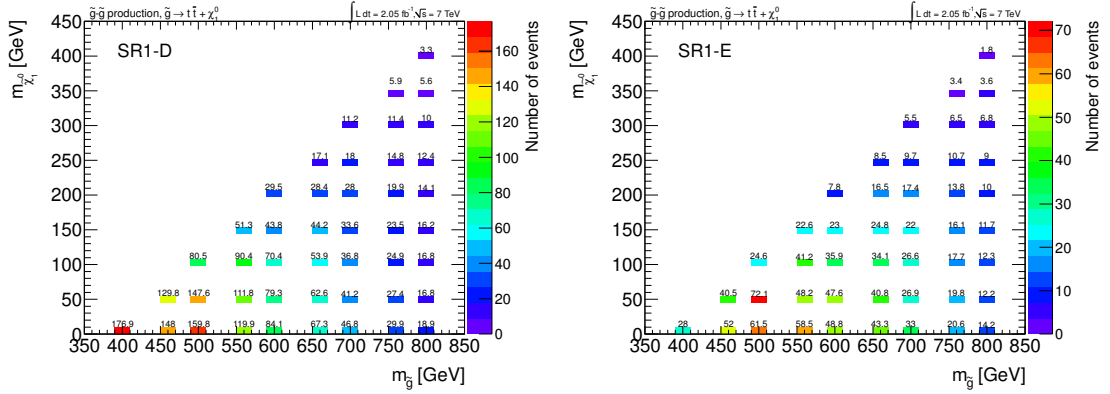
Figure 5.36.: Expected numbers of signal events in the (m_{\tilde{g}}, m_{\tilde{\chi}_1^0}) -plane of the Gt simplified model for an integrated luminosity of 2.05 \text{ fb}^{-1} in SR1-D (left) and SR1-E (right).
