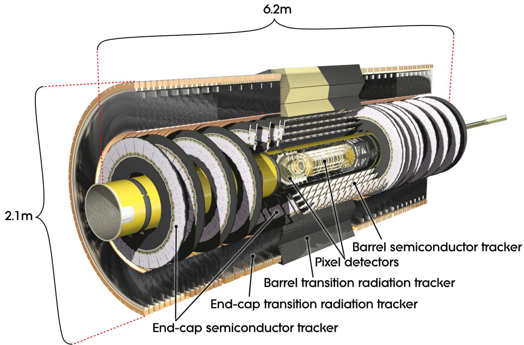
Figure 4.2.: Schematic layout of the ATLAS inner detector [69].
