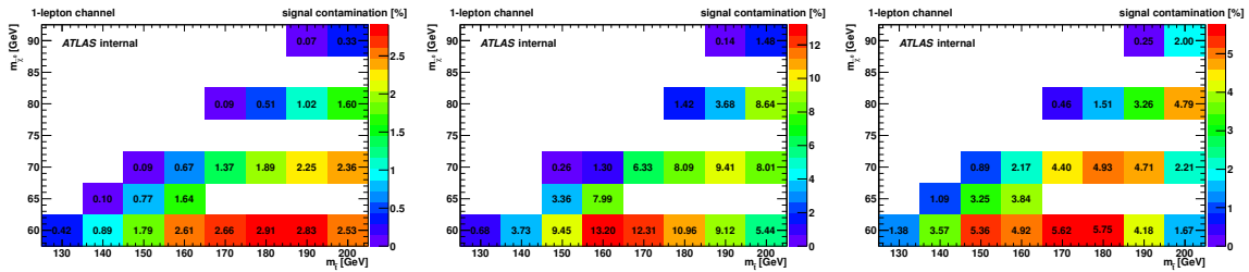
Figure 6.14.: Ratio of the number of expected signal and background events (signal contamination) in the (m_{\tilde{t}}, m_{\tilde{\chi}_1^0}) -plane for the control regions \text{CR}_1^{\text{top}} (left), \text{CR}_2^{\text{top}} (middle) and \text{CR}_1^W (right), respectively.
