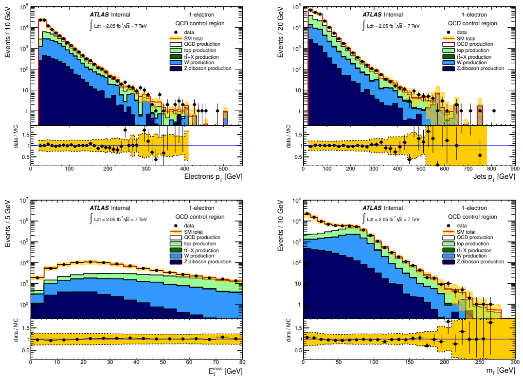
Figure 5.14.: Distributions of the lepton p_T , the p_T of the jets, E_T^{\text{miss}} and m_T for the electron channel. The QCD multijet background is estimated from data. The yellow bands represent the uncertainty on the background prediction and include the uncertainty on the QCD prediction and all the uncertainties on the non-QCD background estimate from Monte Carlo, discussed in Section 5.3.
