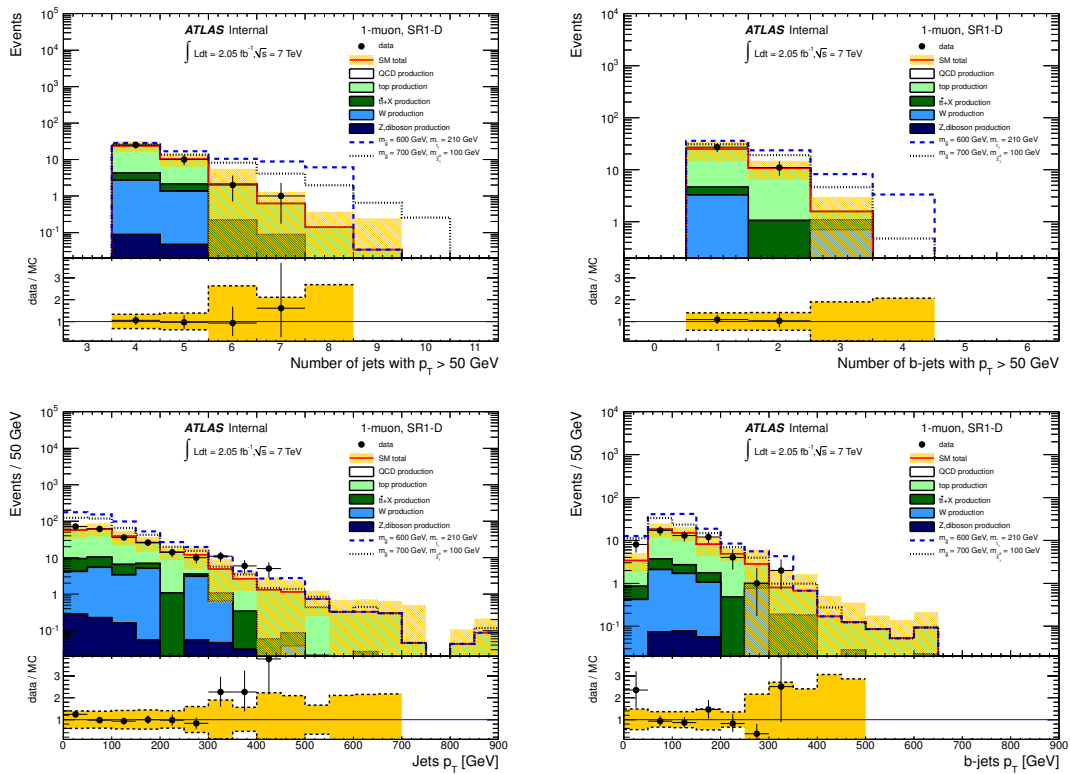
Figure 5.30.: Distributions of the number of jets, the number of b -jets, the jets p_T and the b -jets p_T in SR1-D for the muon channel. The QCD multijet background is estimated from data. The uncertainty on the background prediction includes the uncertainty on the QCD multijet prediction and all the uncertainties on the non-QCD background estimate from Monte Carlo. For reference, two SUSY signals are superimposed, namely one signal point with m_{\tilde{g}} = 600 GeV and m_{\tilde{\chi}_1^0} = 210 GeV and one signal point with m_{\tilde{g}} = 700 GeV and m_{\tilde{\chi}_1^0} = 100 GeV.
