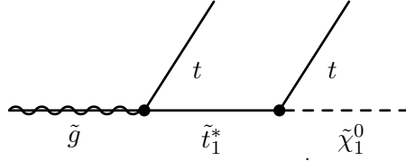
Figure 3.10.: Main gluino decay \tilde{g} \rightarrow tt + E_T^{\text{miss}} in the Gt simplified model.
