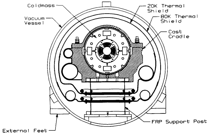
Figure 3. Cross section of IR quadrupole.
