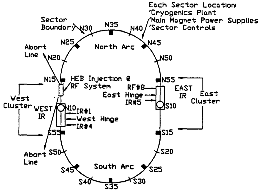
Figure 1. The Super Collider and the Interaction Regions.
