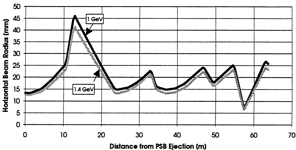
Figure 3: Horizontal beam sizes in the PSB-PS transfer line for the SFT beam at 1 GeV ( \mathcal{E}_x^* = 12.5 \mu\text{m} , \Delta p/p = 0.12\% ) and at 1.4 GeV ( \mathcal{E}_x^* = 12.5 \mu\text{m} , \Delta p/p = 0.29\% ).
