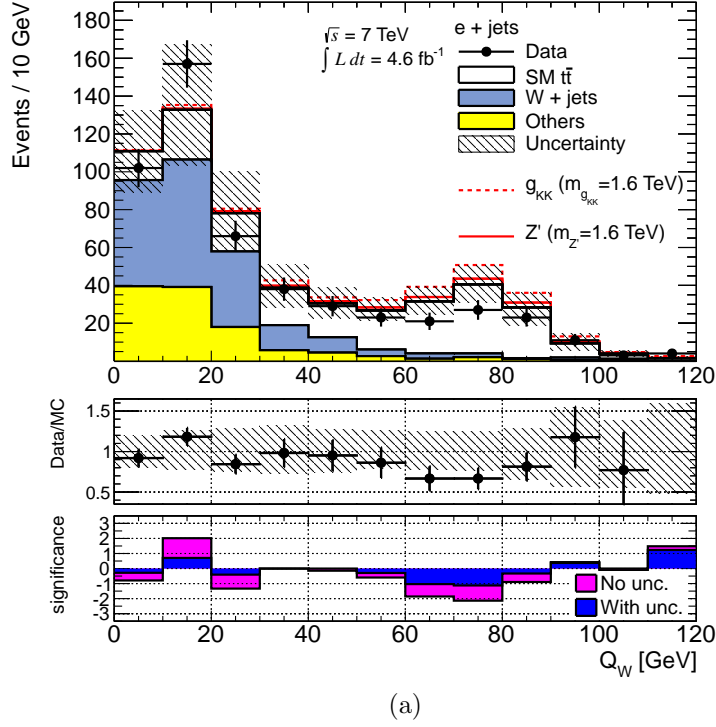
Figure C–2: Reconstructed jet Q_W value of the hadronic top candidate in the e+jets (a) and the \mu +jets (b) channels, after the final selection of events, except the requirements on the candidates reconstructed mass and Q_W observables. The uncertainty corresponds to the (bin by bin) quadratic sum of all sources of uncertainties (including the statistical uncertainty of the MC samples) considered in the analysis. The statistical significance of the difference between data and the predicted background is shown in the bottom inset. Hypothetical signals (a Z' with m_{Z'} = 1.6 TeV and a g_{KK} with m_{g_{KK}} = 1.6 TeV) are shown on top of the expected Standard Model background.
