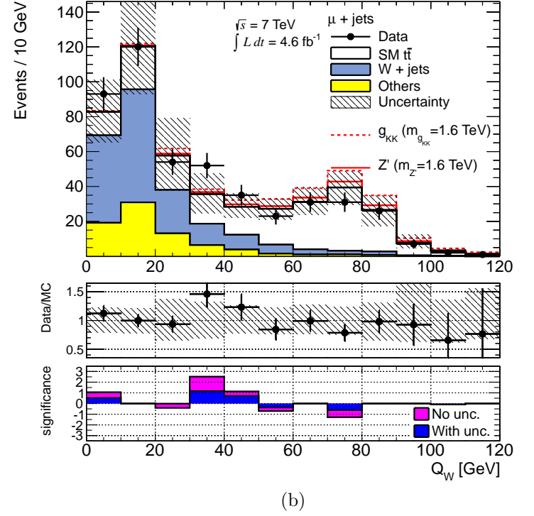
Figure C–2: Reconstructed jet Q_W value of the hadronic top candidate in the e+jets (a) and the \mu +jets (b) channels, after the final selection of events, except the requirements on the candidates reconstructed mass and Q_W observables. The uncertainty corresponds to the (bin by bin) quadratic sum of all sources of uncertainties (including the statistical uncertainty of the MC samples) considered in the analysis. The statistical significance of the difference between data and the predicted background is shown in the bottom inset. Hypothetical signals (a Z' with m_{Z'} = 1.6 TeV and a g_{KK} with m_{g_{KK}} = 1.6 TeV) are shown on top of the expected Standard Model background.
