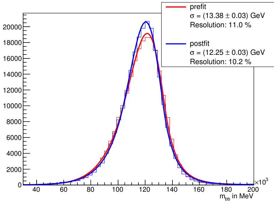
Figure 4.1: m_{bb} after implementing the kinematic fit in Overkill without m_H constraint yields an 8 % improvement. If the m_H = 91.2 GeV constraint is added, the width is \sigma = (12.31 \pm 0.03) GeV.
