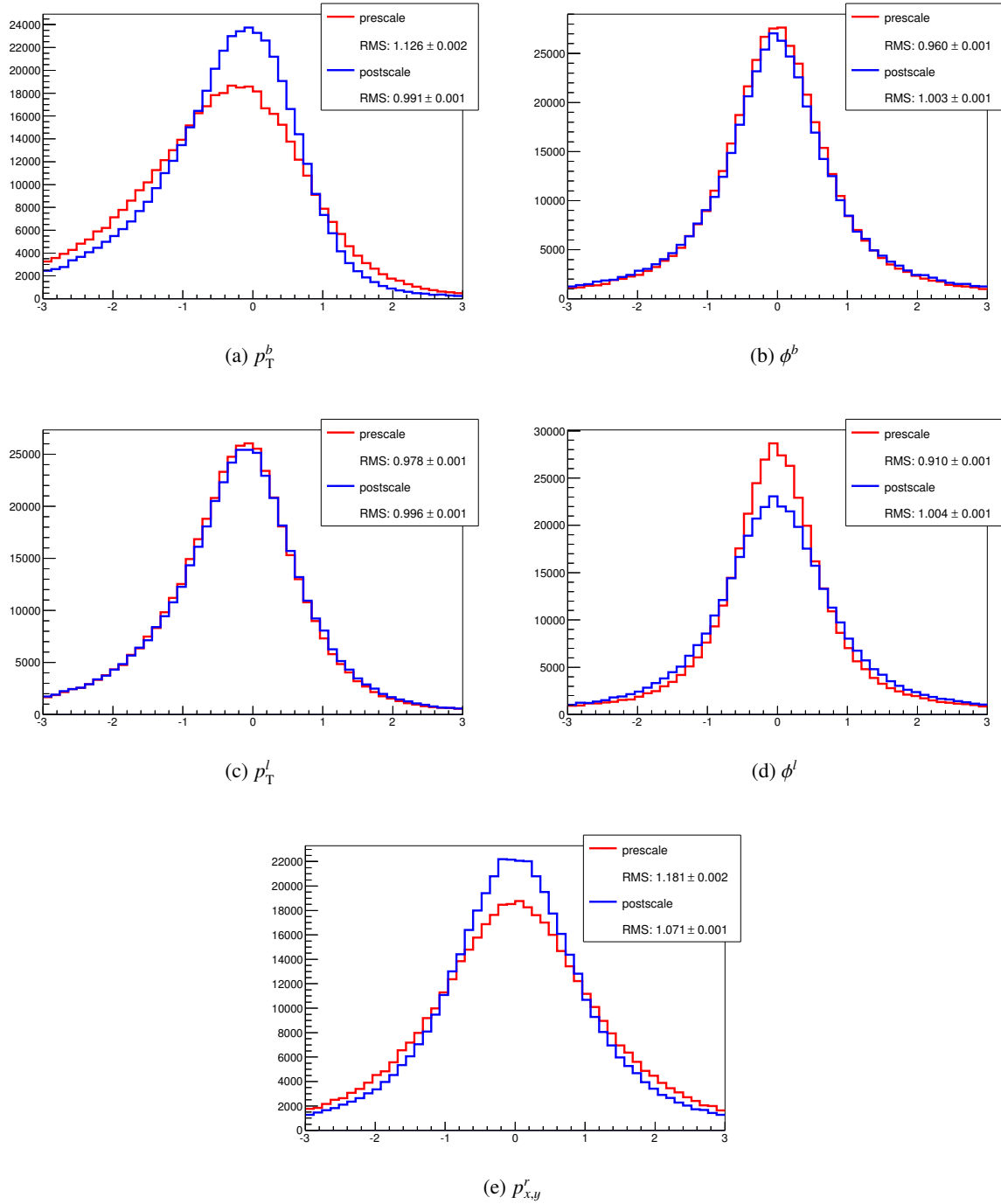
Figure A.2: Pulls g_{tr} for the kinematic variables when fitting without m_Z constraint.
