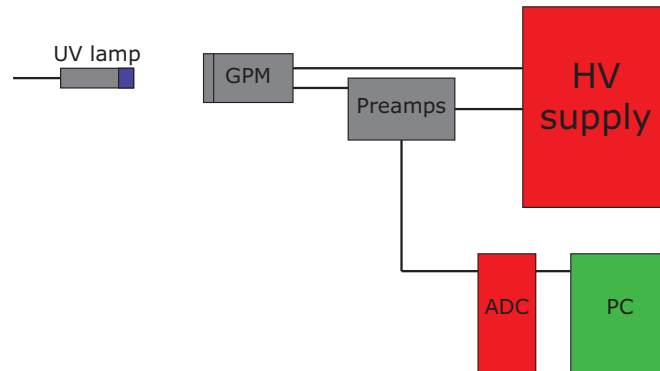
Figure 7.2: Experimental setup. A Hg(Ar) lamp provides the UV photons producing the signals, preamplified with Cremat CR-111 preamplifiers and digitised with a CAEN N1728B NIM ADC module.
