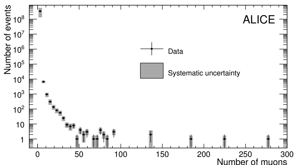
Figure 7.1: Muon multiplicity distribution of the whole sample of data (2010-2013) corresponding to 30.8 days of data taking.
