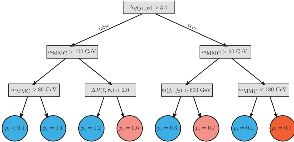
Figure 7.1: Simplified example of a single decision tree with N_{\max} = 3 . In addition to events in the leaf node with the highest signal purity p_s = 0.9 , also events in other nodes with p_s > 0.5 are considered signal-like.
