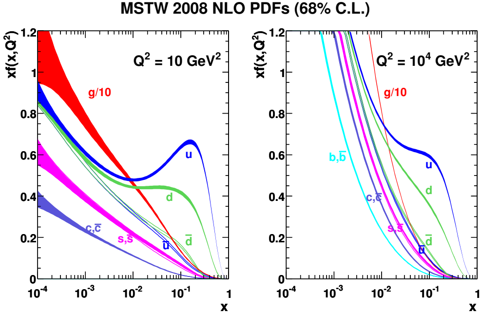
Figure 2.9: Parton-distribution-functions and uncertainties at 68% confidence level for momentum transfers of Q^2 = 10 \text{ GeV}^2 (left) and Q^2 = 10^4 \text{ GeV}^2 (right) [36].
