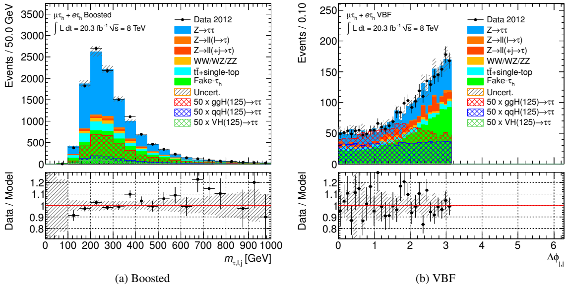
Figure D.1: Distributions of the jet-related input observables for the training of the de-correlated BDTs in the (a) Boosted and (b) VBF category. The background components are estimated with the techniques described in section 7.4.
