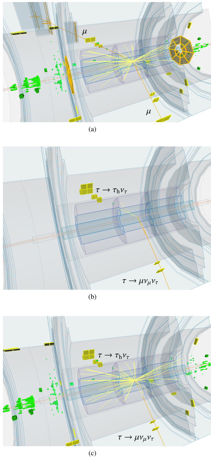
Figure 5.6: The embedding method applied to an example event in a schematic view of the ATLAS detector. Starting from a Z \rightarrow \mu\mu decay selected from data (a), a Z \rightarrow \tau\tau \rightarrow \mu\tau_h\nu_\tau decay with identical kinematics but no pile-up (b) is simulated and then merged with the original data event (c), from which the muons have been removed beforehand.
