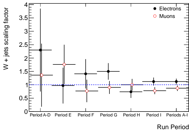
Figure 5.5: W + \text{jets} scaling factor for the different data taking periods, determined in the W control region. The factor is obtained by subtracting the other simulated backgrounds from the data and then dividing by the expected number of W + \text{jets} events. Only the statistical errors are shown and indicate consistence between the runs. The periods correspond to the following integrated luminosities: 0.3 (A-D), 0.9 (E), 1.7 (F), 5.7 (G), 7.0 (H) and 19.0 \text{ pb}^{-1} (I) totaling 34.6 \text{ pb}^{-1} .
