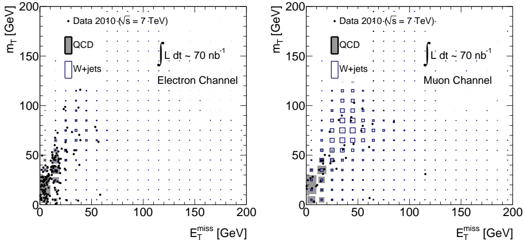
Figure 4.2: E_T^{\text{miss}} versus m_T plane for background normalization of QCD multi-jet and W + \text{jets} events in the electron (left) and muon (right) channel. The size of the boxes reflects the relative magnitude of each contribution.
