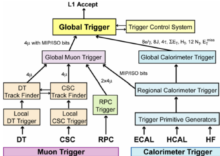
Figure 2.2: CMS L1 trigger flow chart.
