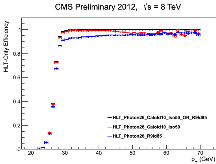
Figure 4.4: HLT efficiency as a function of reconstructed photon p_T for the HLT leg with E_T = 26 GeV cut.
