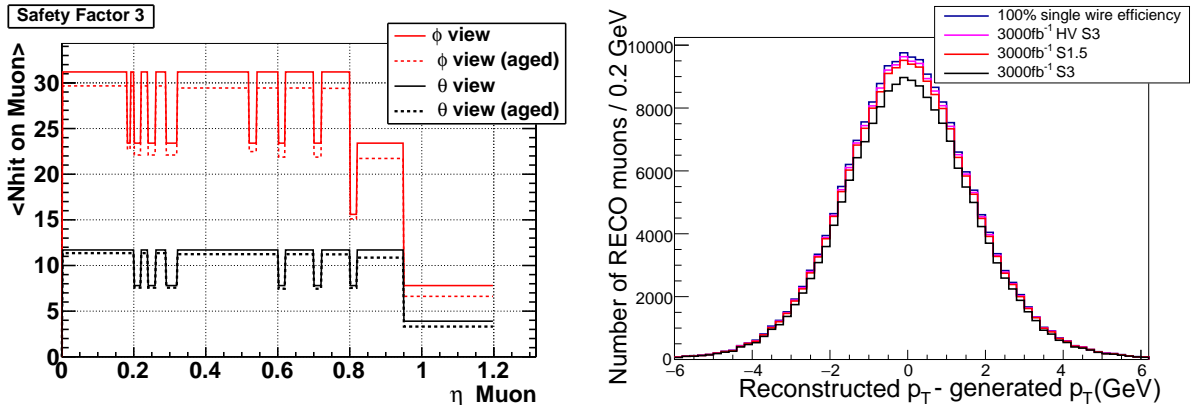
Figure 3.9: Left: Number of DT hits per high p_T muon track as a function of \eta for a perfect detector (full lines) in both the \phi (red) and \theta measurement planes. The dash lines show the impact of aging in a scenario described in the text. Right: reconstructed p_T using the standalone muon algorithm in a simulation of 100 GeV muons with different detector scenarios for detector aging: a perfect detector (blue line), the aging scenario described in the text (pink line), the effect of maintaining the HV constant at 3550 V (black line) and the effect of reducing the safety factor to 1.5 in the latter scenario (red line).
