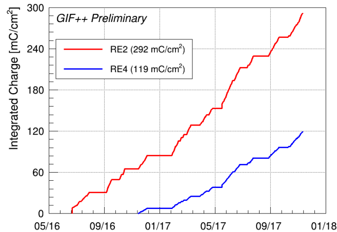
Figure 5.4: Integrated charge versus time collected during the GIF++ studies for the RE2/2 and RE4/2 chambers. The RE4/2 chamber has been turned on few months later because of total gas flow limitations. Different slopes account for different attenuation factors during data taking.
