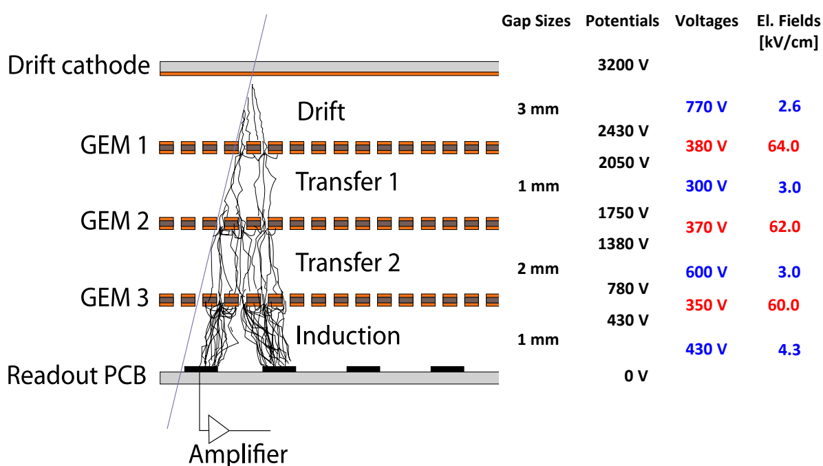
Figure 6.13: Principle of operation of a generic triple-GEM chamber and definition of drift, transfer, and signal induction gap regions within the detector [86]. The columns on the right give the actual gap sizes in the detector. They also list typical values for electric potentials on the seven electrodes and typical values for voltages and electric fields across the four gaps (blue) and the three foils (red) if the nominal potential of 3200 V in Ar/CO 2 70:30 is applied to the drift cathode, i.e. for operation at the start of the efficiency plateau.
