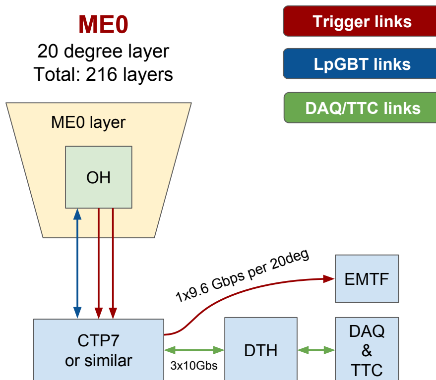
Figure 6.45: Diagram of the ME0 electronics readout system.
