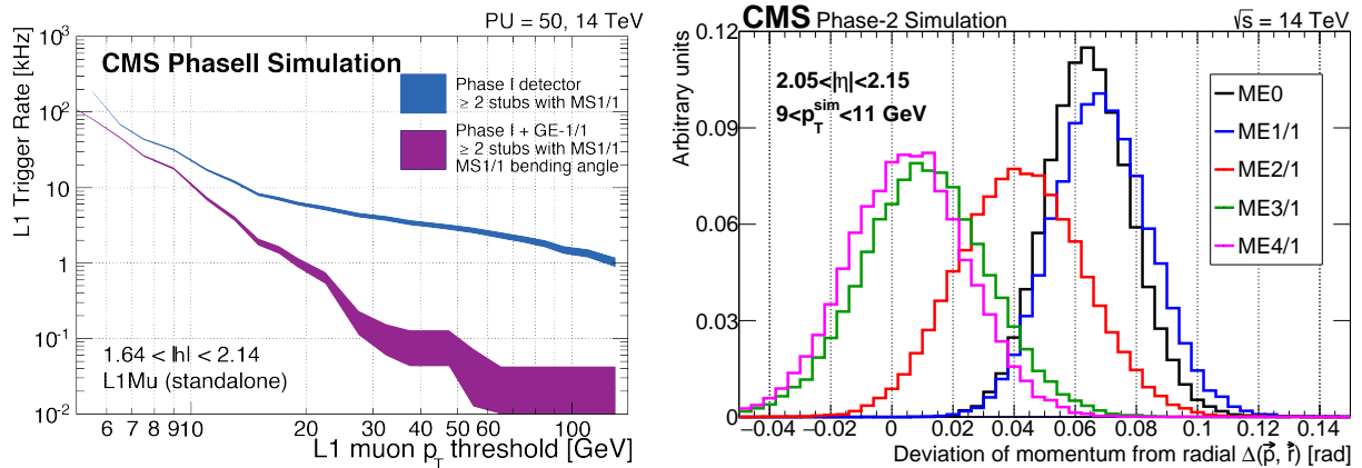
Figure 6.2: Left: Trigger rate reduction with the deployment of muon direction measurement using GEM GE1/1 and CSC ME1/1 chambers [7]. Right: The distribution of local directions for muons with p_T = 10 GeV in each of the four muon stations shows that the use of directions in the first two stations can be effective in rejecting low transverse momentum muons [24]. In far stations, the “unbending” of muons due to the radial component of the magnetic field and substantial multiple scattering reduce effectiveness of the direction measurement for rejection of low transverse momentum muon candidates.
