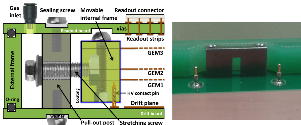
Figure 6.14: Left: Cross-section through inner and outer module frames and GEM foils that shows how the GEM foils are mounted within a CMS triple-GEM module so that they can be mechanically tensioned against the pull-out posts without deforming the drift or readout boards. Right: Stainless steel pull-out post and spring-loaded pins that are soldered to the drift board for making electrical HV connections to corresponding contact pads on the GEM foils.
