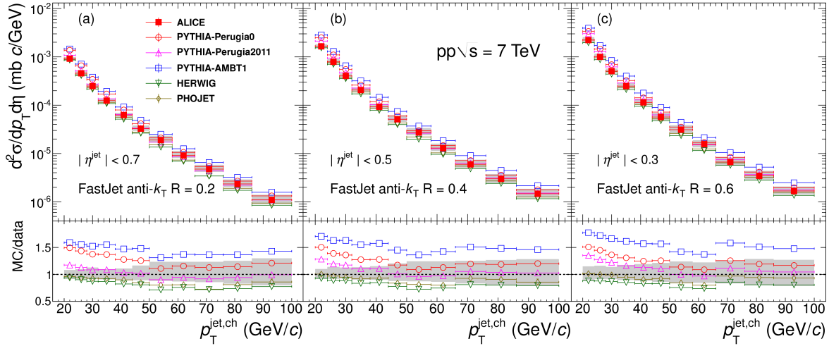
Figure 8.5: Comparison of jet spectrum from proton-proton collision at \sqrt{s} = 7 TeV with Monte-Carlo predictions produced by PYTHIA tune AMBT1 (blue squares), Perugia-0 (red circles), Perugia-2011 (magenta up-triangles), HERWIG (green down-triangles) and PHOJET (brown diamonds).
