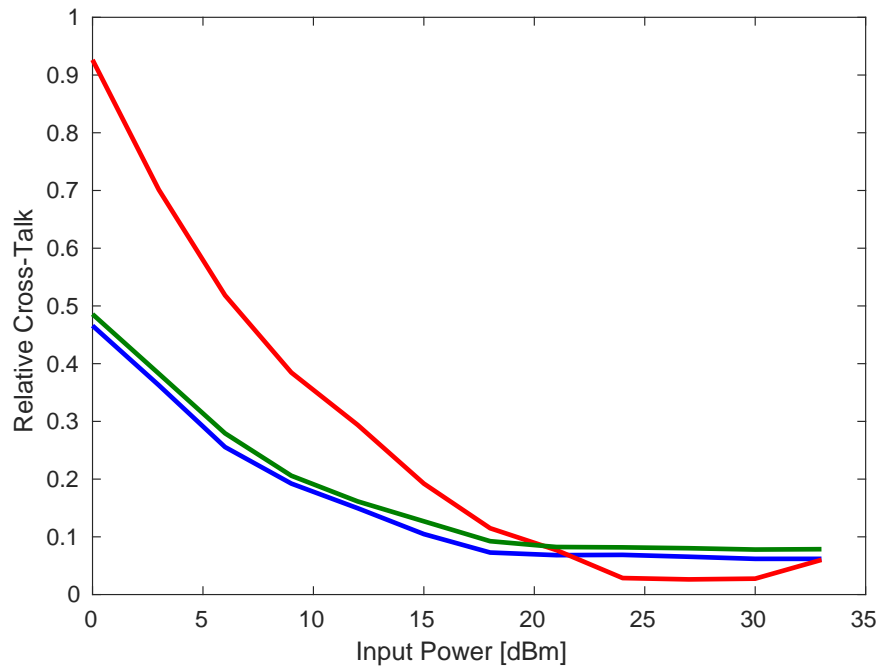
Figure 3.27: Dependence of the relative amplitude of cross-talk on the diode versus the input power. Blue: Diode 1, Red: Diode 2 and Green: Diode 3.
