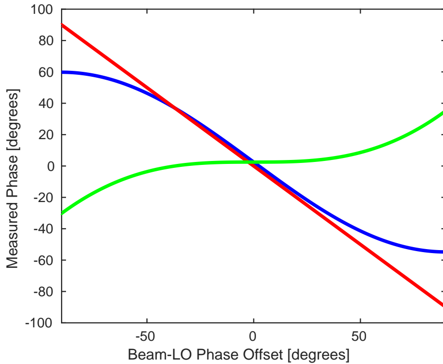
Figure 5.21: Difference (green) between a phase reconstruction method using the small angle approximation (blue), and the full reconstruction method taking into account non-linearities in the mixer output for large phase offsets (red).
