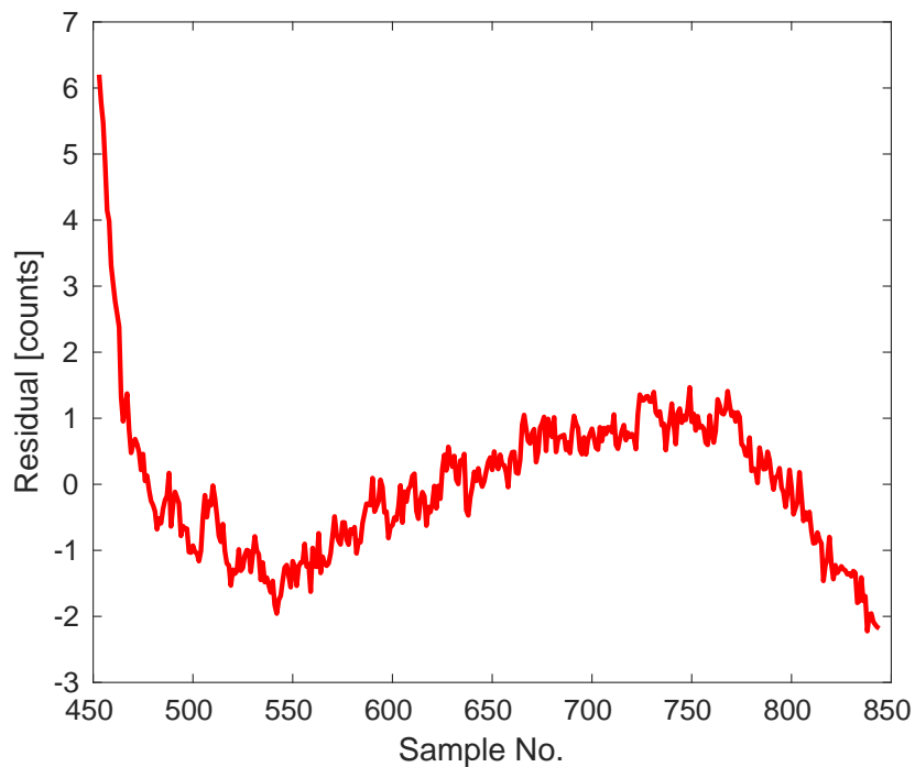
Figure 5.7: Residuals between the measured diode output and the exponential fit to the droop shown in Figure 5.6. Sampled at 357 MHz (2.8 ns per sample).
