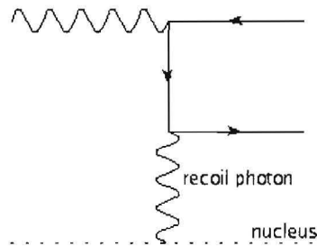
Figure 2.2: Feynman diagram of photon pair production.
