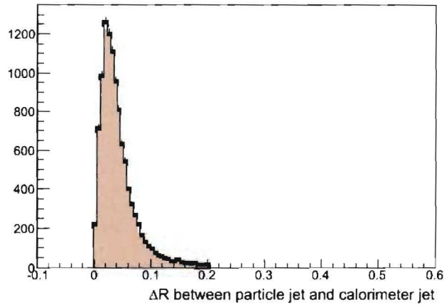
Figure 5.19: \Delta R between the true particle level jet and the signal jet. Signal jets which are not matched to a particle level jet within \Delta R < 0.2 are not considered.
