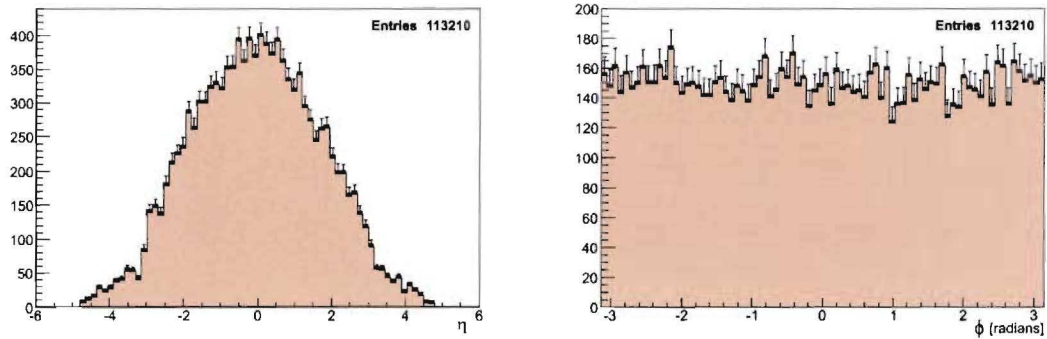
Figure 5.14: \eta (left) and \phi (right) distributions for jets in the CSC datasets which pass the signal selection cuts (see text for more details on the cuts).
