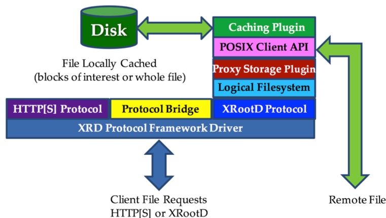
Figure 2. The caching server architecture with the major components.
