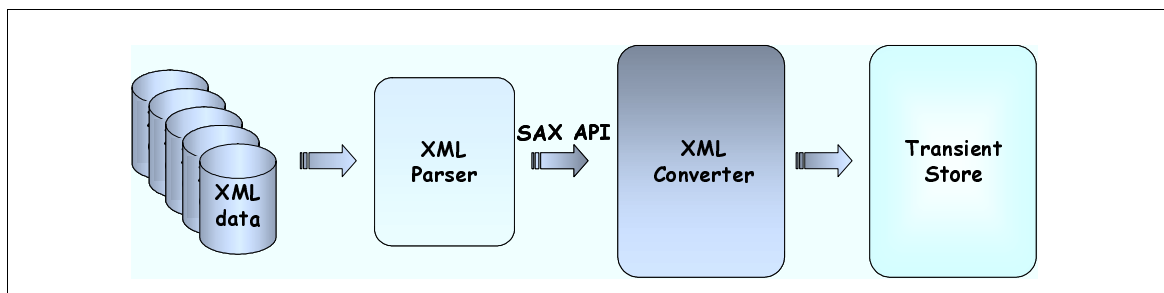
Figure 2.10 Conversion process for XML based data in Gaudi detector description framework
