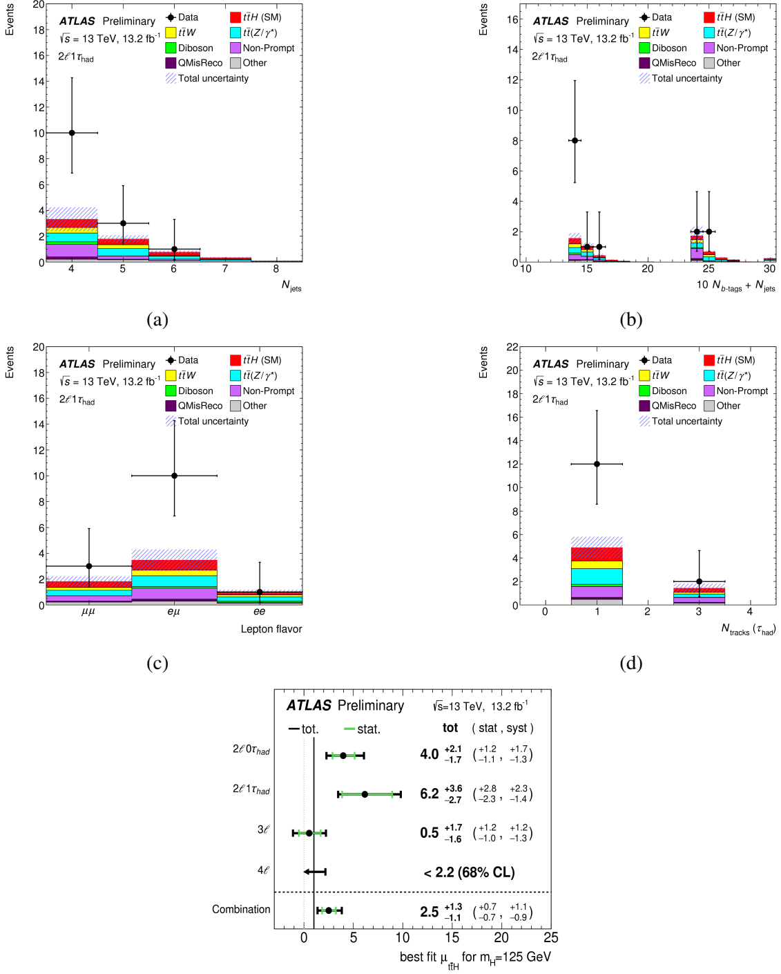
Figure 1: Characteristics of selected events in the SR: (a) number of jets; (b) 10 \times the number of b-tagged jets plus the total number of jets; (c) lepton flavor composition; (d) number of \tau_{\text{had}} tracks. The background expectation is pre-fit (using initial values of the background systematic uncertainty nuisance parameters) and the signal is set to one to the Standard Model (SM) expectation. The hatched region shows the total uncertainty on the background plus the SM signal prediction in each bin. (e) The best-fit value of the signal strength \mu_{t\bar{t}H} of all the multilepton final states and combined. The SM prediction is \mu_{t\bar{t}H} = 1 [3].
