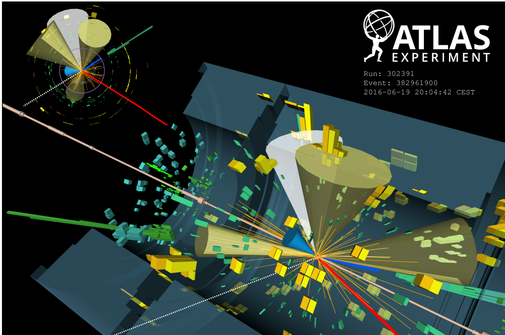
Figure 2: Event display of one of the candidate event in 2\ell 1\tau_{\text{had}} . The blue track is the selected electron; the red track is the selected muon; the white cone is the \tau_{\text{had}} candidate; the three yellow cones are the selected jets and azure cone is the selected b-tagged jet. The green and yellow bars indicate the energy deposits in the electromagnetic and hadronic calorimeters [3].
