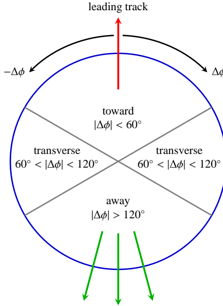
Figure 6: Definition of UE regions as a function of the azimuthal angle with respect to the leading track [12].
