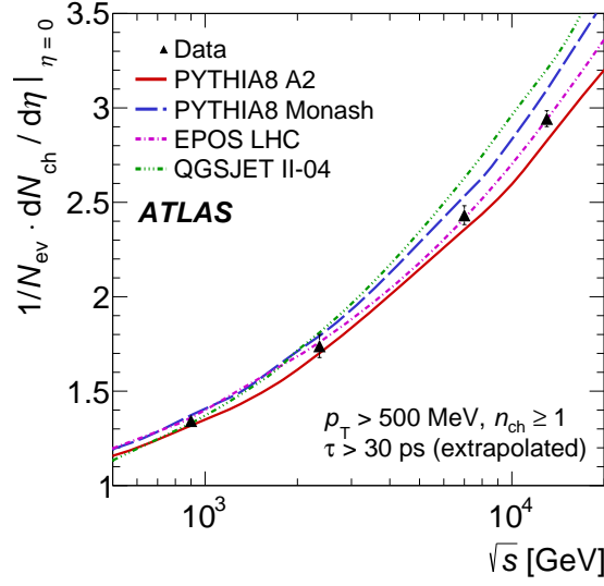
Figure 5: The average primary charged-particle multiplicity in pp interactions per unit of pseudorapidity for |\eta| < 0.2 as a function of the centre-of-mass energy [6].
