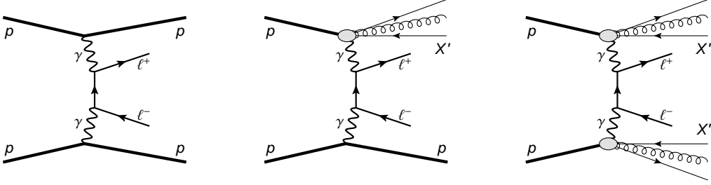
Figure 11: Schematic diagrams for exclusive (left), single-proton dissociative (middle) and double-proton dissociative (right) two-photon production of lepton pairs in pp collisions [14].
