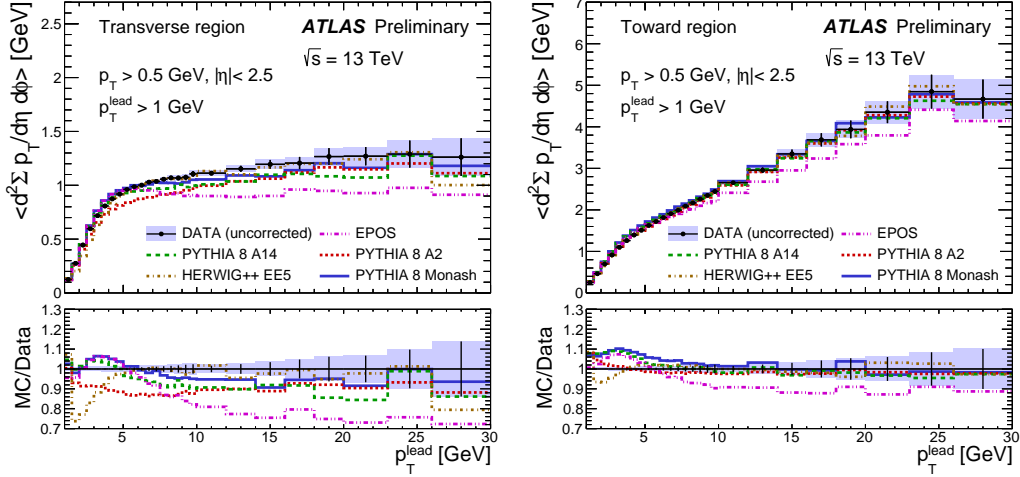
Figure 8: Comparison of detector level data and MC predictions for average scalar p_T sum density of tracks as a function of leading track transverse momentum, p_T^{\text{lead}} , in the transverse (left) and toward (right) regions [12].
