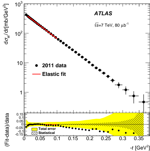
Figure 2: A fit of the theoretical prediction with \sigma_{\text{tot}} and B as free parameters to the differential elastic cross-section [2].
