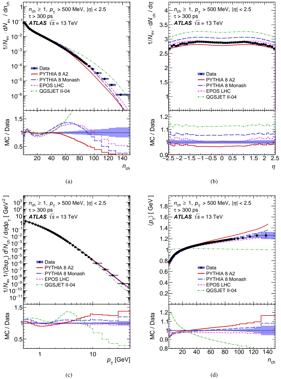
Figure 4: The primary charged-particle multiplicity distribution (a), the multiplicity as a function of (b) pseudorapidity, and (c) transverse momentum; and (d) the mean transverse momentum, \langle p_{\text{T}} \rangle , versus particle multiplicity [6].
