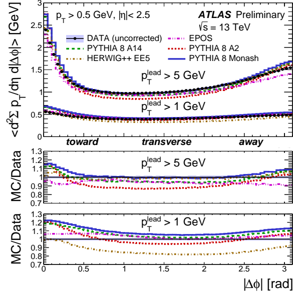
Figure 7: Comparison of detector level data and MC predictions for the |\Delta\phi| distributions of average scalar p_T sum density of tracks [12].
