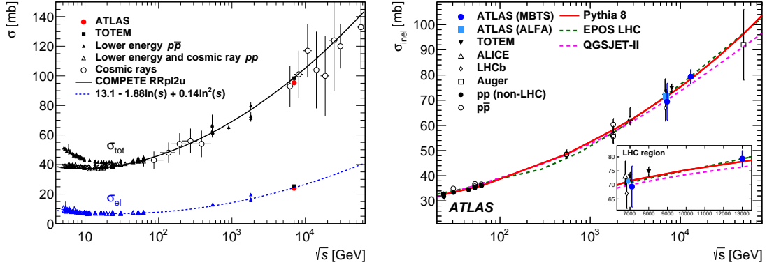
Figure 3: Left, the comparison of total and elastic cross-section measurements presented here with other published measurements and model predictions as a function of the centre-of-mass energy [2]. Right, the inelastic proton-proton cross-section versus \sqrt{s} [5].
