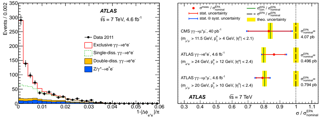
Figure 12: Di-electron acoplanarity distribution (left) after the selection requirements. The exclusive and single-dissociative yields are determined from the fit. On right, comparison of the ratios of measured (red points) and predicted (solid green lines) cross-sections to the uncorrected EPA calculations (black dashed lines). Results for the muon and electron channels are also compared with a similar CMS measurement. The yellow band represents the theoretical uncertainty of 1.8% (1.7%) on the predicted (uncorrected EPA) cross-section [14].
