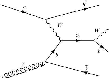
Figure 1: Leading-order Feynman diagram of single Q ( Q = T, Y ) production in Wb fusion and subsequent decay into Wb .
