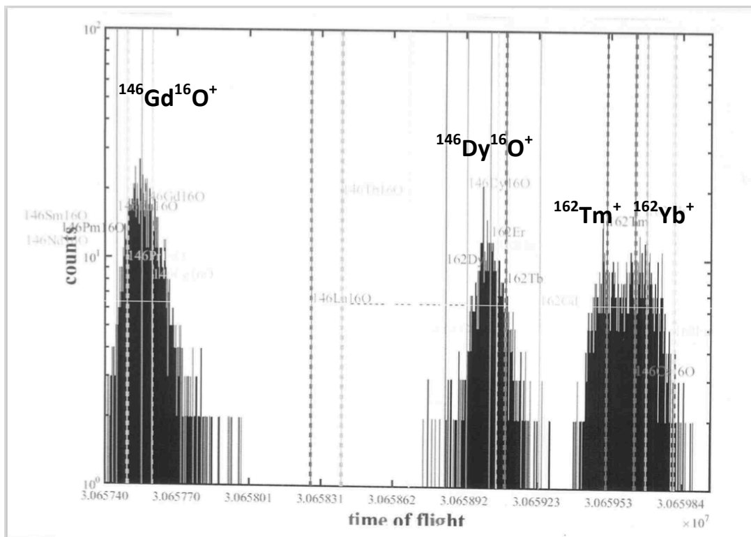
Fig.4 MR-TOF spectrum for the oxides (mass 162). Due to the absence of ^{146}\text{Eu}^{16}\text{O}^+ , ^{146}\text{Gd}^{16}\text{O}^+ has a purity of the order of 45%.
