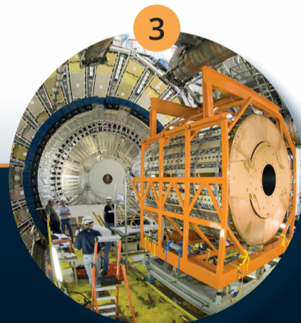
Inner Detector measures the momentum of each charged particle
