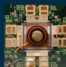
Inner Detector measures the momentum of each charged particle
