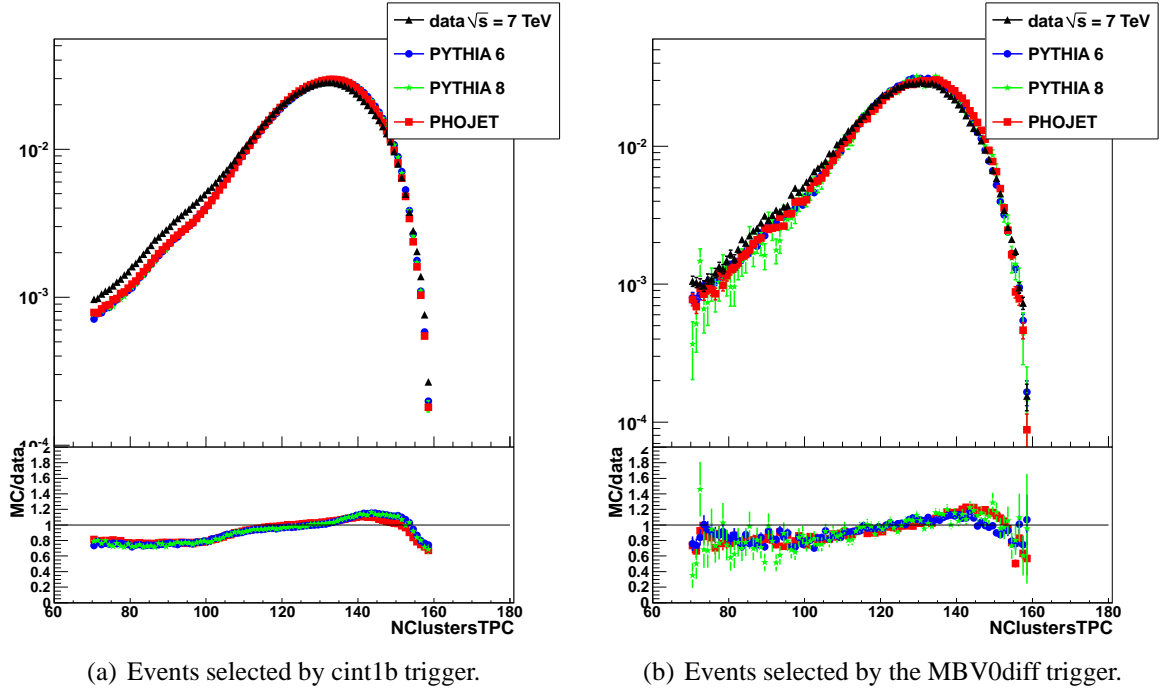
Figure 6.4: Distributions of number of TPC clusters. The bottom panel shows the ratio of MC and data.
