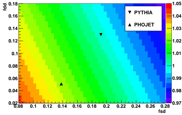
(a) PYTHIA 6
