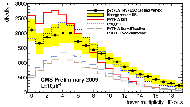
Figure 9: Distribution of accepted events as a function of N_{HF+} .
