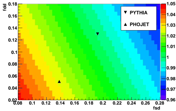
(c) PYTHIA 8
