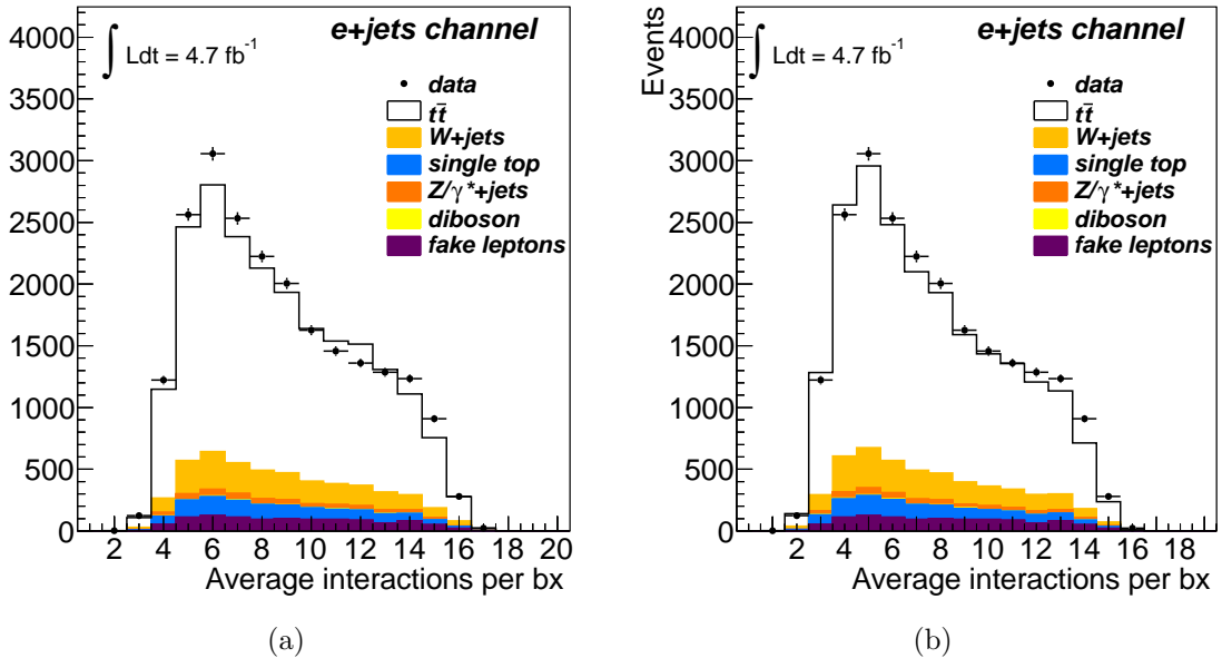
Figure 6.14: a) Average number of interactions per bunch crossing, a) before, and b) after reweighting, in the e+jets channel.
